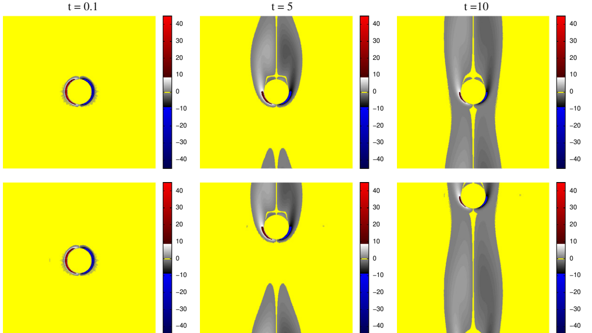
Fig. 13. (Color online) Snapshots of vorticity at different time instants for configuration ‘fixed’ (top) and ‘moving’ (bottom).
