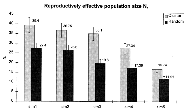
Figure 6. — Reproductively effective population size N_r in 5 scenarios with the 2 different stand structures “Random” and “Cluster”.
