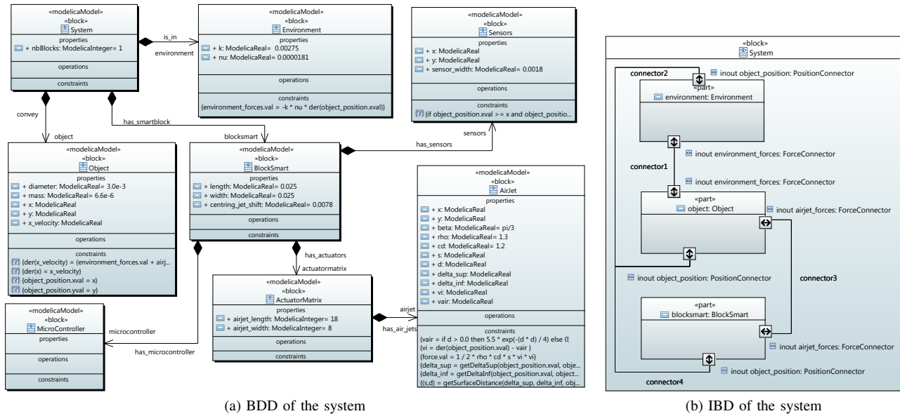
Fig. 3: SysML model of the system
