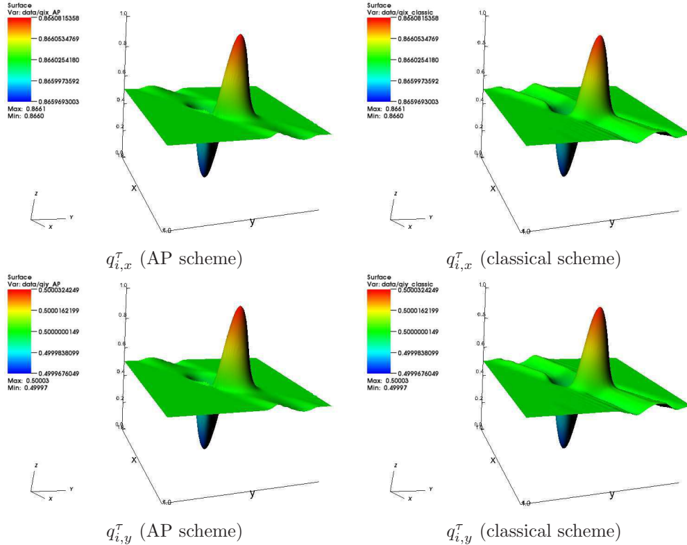
FIGURE 4. Resolved case at time t = 6 \times 10^{-6} : x and y components of the ion momentum \mathbf{q}_i^{\tau} as functions of (x, y) computed with the AP scheme (left) and the classical scheme (right).
