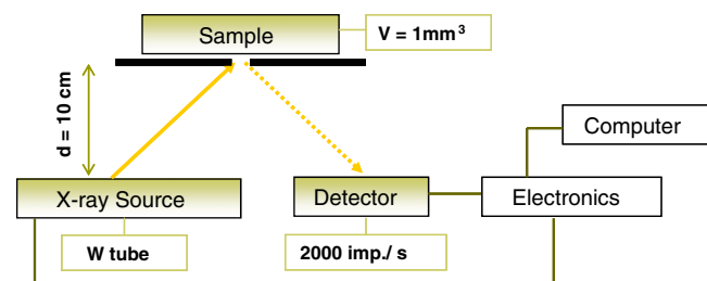
Fig. 3. Schematic of the EDXRF device. X-rays from the tungsten tube pass through a hole on their way to the sample. X-rays from the sample then travel to the “2000 impulsions per second” detector. The signal at the detector is then processed by electronics and sent to a computer for analysing the spectra.
