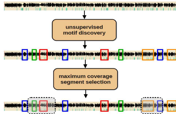
Figure 1: The different steps involved in motif discovery based on thumbnail generation: motifs occurrences are indicated with colored rectangles, selected segments are highlighted in shadowed rounded boxes. Pale green regions below the waveform indicate silences.
