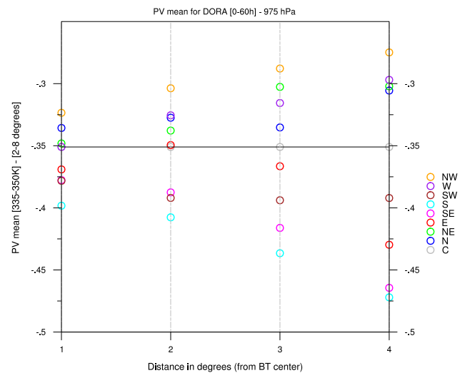
FIG. 3. Mean PV values averaged over a 60-h period, a 335-350-K layer and a 200-800 annulus region surrounding the storm predicted center, for experiments initialized with a 975 hPa central pressure.
