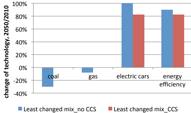
Fig.17. Technology roadmaps by least changed energy mix in the US in 2050 compared to 2010
