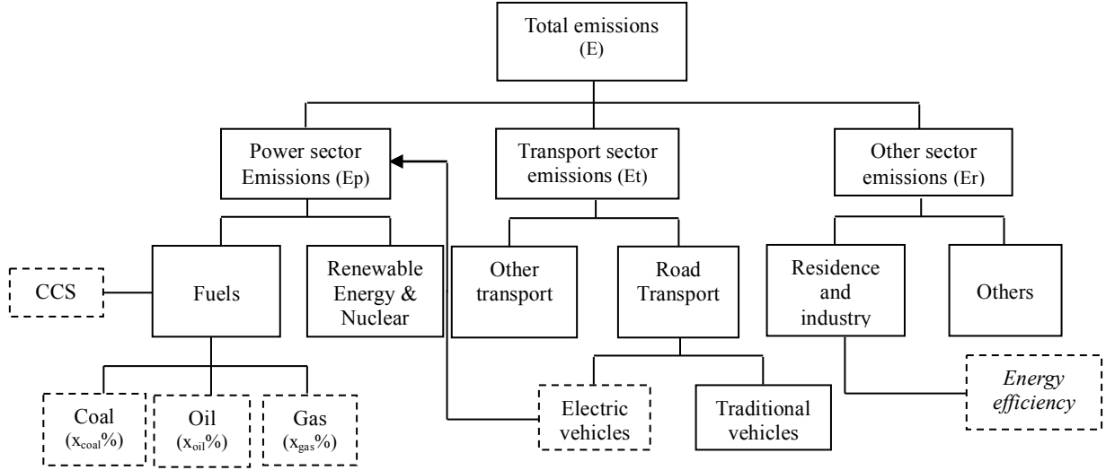
Fig.2. Schema of Sectoral Emission Model
