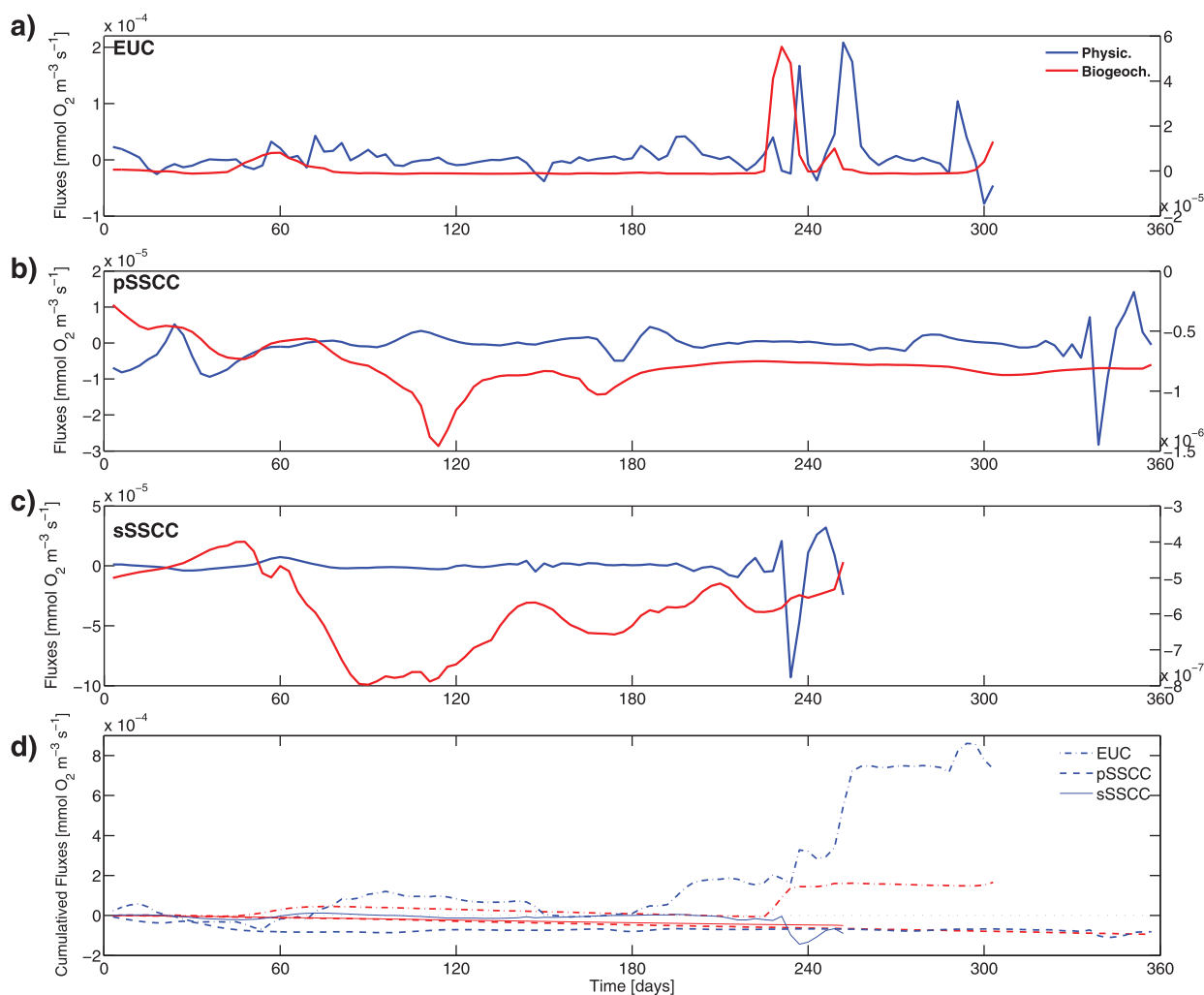
Figure 6. O 2 budget along the main paths of the ECS: evolution of the relative contribution of the physical (blue lines) and biogeochemical (red lines) processes to the O 2 changes along the float pathways of the (a) EUC, (b) the pSSCC, and (c) the sSSCC. The left (right) scale is for the physical (biogeochemical) process. Evolution of Figure 6d, the cumulative contribution of the physical (blue lines) and biogeochemical (red lines) processes to the rate of O 2 change along the paths. In Figure 6d, the dash-dotted, dashed, and solid lines indicate the EUC, pSSCC, and sSSCC, respectively. This scheme is representative for both ROccam and RSoda solutions.
