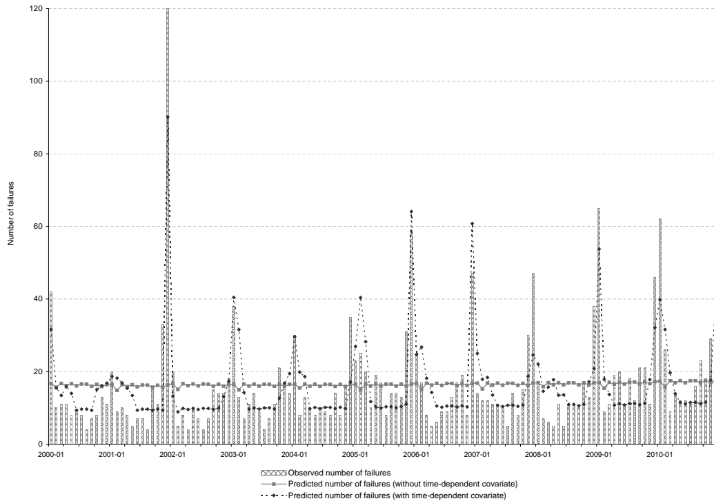
FIGURE 4. Comparison of the monthly numbers of failures observed and estimated using LEYP models with and without time dependent covariate, on the whole CUB network
