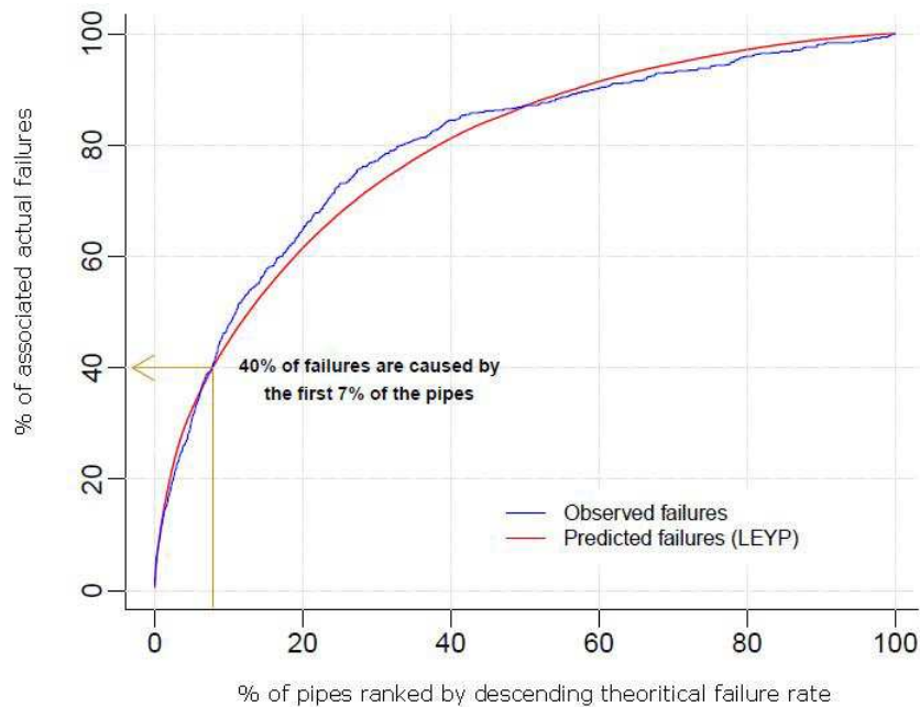
FIGURE 5. Percentage of breaks associated to the pipes according to the model and the observations
