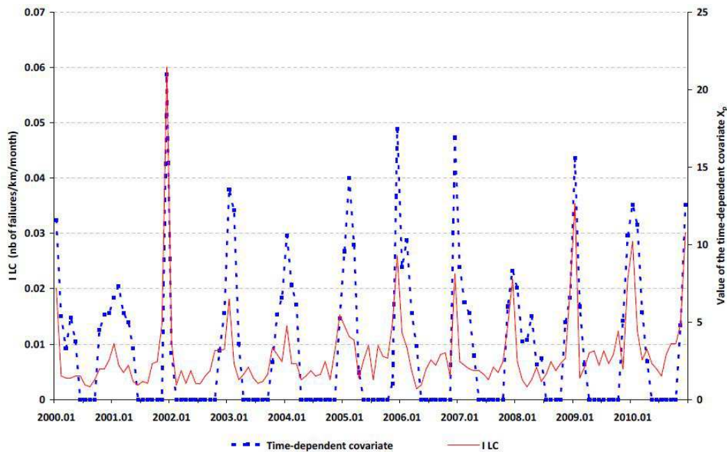
FIGURE 3. Linear indicator of failure (ILC) and time-dependant covariate - CUB data between 2000 and 2010
