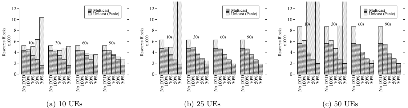
Figure 4: Average resource blocks employed at eNB to reach 100% dissemination. Note that even few panic zone retransmissions (in unicast) result very costly in resources.
