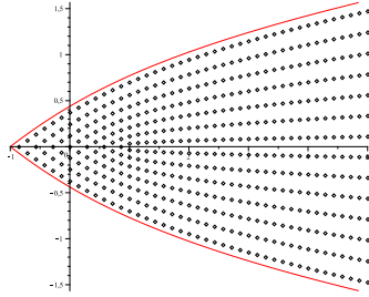
FIGURE 1. Semiclassical joint spectrum of the Jaynes-Cummings model.
