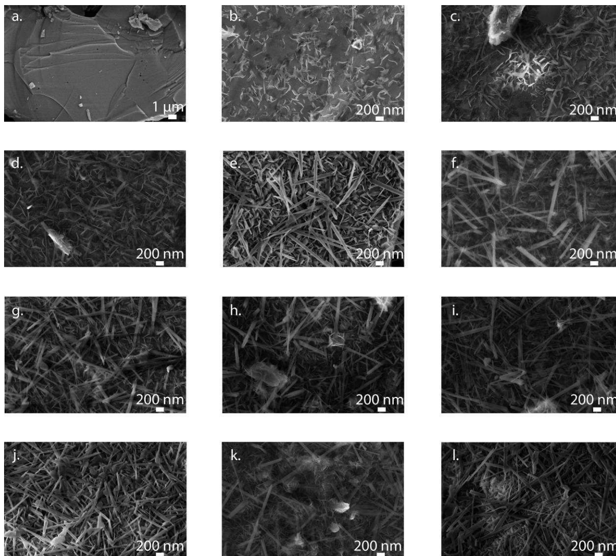
Figure S3: SEM micrography, in InLens mode, of \text{La}_{1.5}\text{Mg}_{0.5}\text{Ni}_7 sample (a;) non corroded and corroded for (b.) 6h, (c.) 24h, (d.) 48h, (e.) 4 days, (f.) 1 week, (g.) 2 weeks, (h.) 4 weeks, (i.) 6 weeks, (j.) 8 weeks, (k.) 12 weeks, and (l.) 16 weeks
