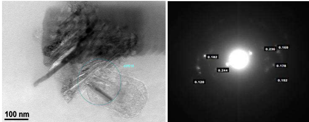
Figure S6: TEM bright field micrograph and electronic diffraction pattern related to the circle, for the sample \text{La}_{1.5}\text{Mg}_{0.5}\text{Ni}_7 corroded for 8 weeks in 8.7M KOH . Interplanar distances are indicated on the diffraction pattern.
