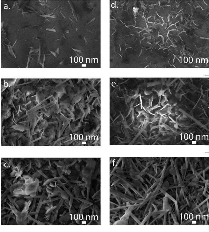
Figure 5: SEM micrographs at magnification 50k, in InLens mode, of La 2 Ni 7 sample corroded for (a.) 6h, (b.) 48h and (c.) 8 weeks on the left and La 1.5 Mg 0.5 Ni 7 sample corroded for (d) 6h, (e.) 48h and (f) 8 weeks on the right.
