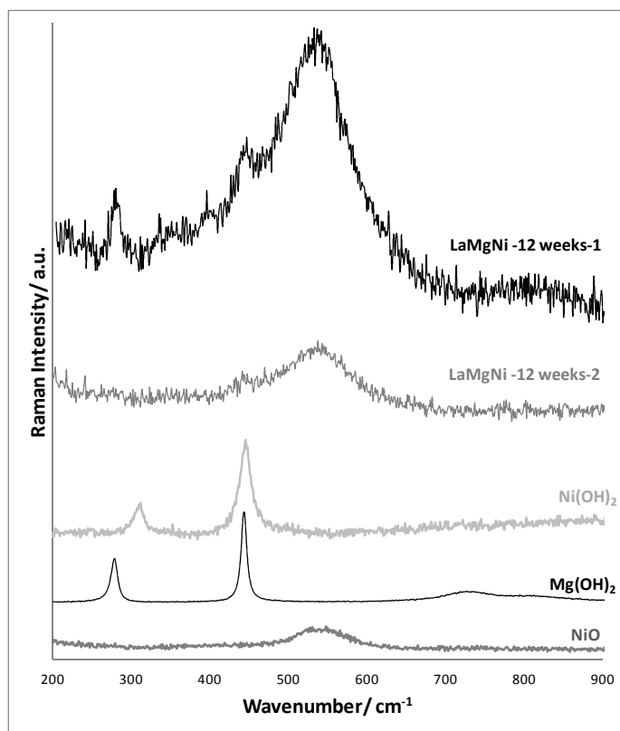
Figure S4: Raman spectra of \text{La}_{1.5}\text{Mg}_{0.5}\text{Ni}_7 sample corroded for 12 weeks compared to \text{Ni}(\text{OH})_2 , \text{NiO} and \text{Mg}(\text{OH})_2 references. Acquisition conditions : 600sec.
