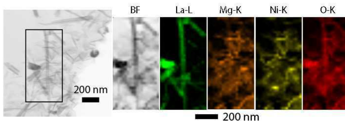
Figure 8: TEM micrograph and EDS-STEM elemental mapping of La, Mg, Ni and O on \text{La}_2\text{Mg}_{0.5}\text{Ni}_7 sample corroded 48h in 8.7M KOH.
