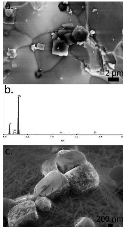
Figure 11: a. SEM micrograph and b. SEM-EDS analysis on \text{La}_2\text{Mg}_{0.5}\text{Ni}_7 sample non-corroded, focusing on cubic crystal of MgO. c. SEM micrograph showing MgO crystals being transformed into \text{Mg}(\text{OH})_2 in the \text{La}_2\text{Mg}_{0.5}\text{Ni}_7 sample corroded 48 hours in 8.7M KOH.
