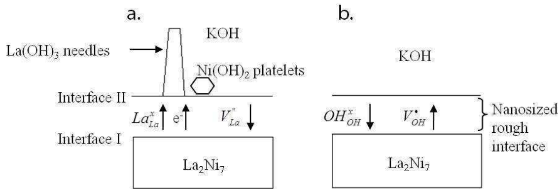
Figure 12: Corrosion mechanisms by a. cationic and b. anionic transport as proposed by Maurel et al. [6], modified (this work) to introduce the presence of the \text{Ni}(\text{OH})_2 platelets.
