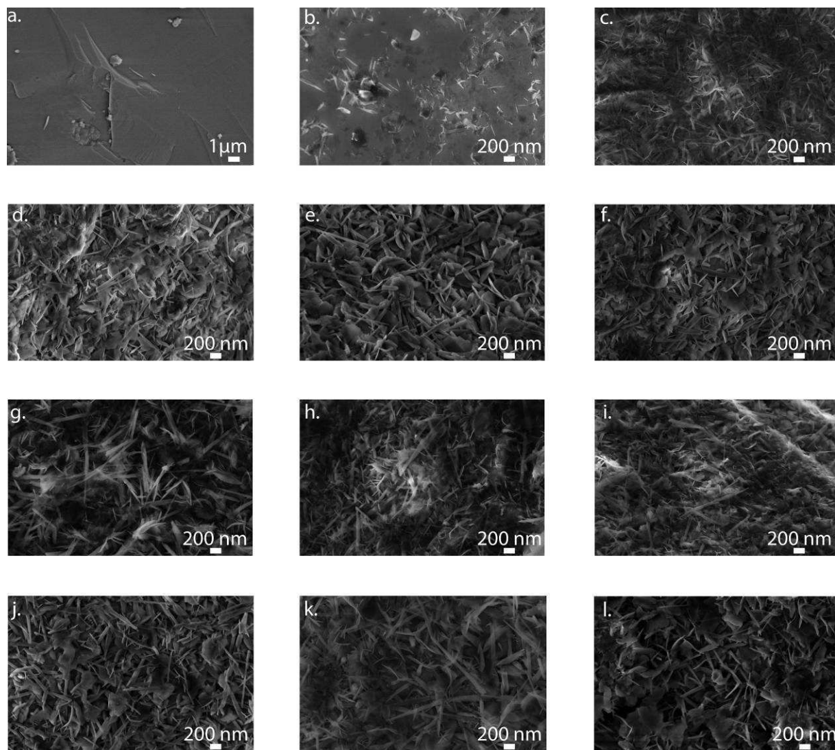
Figure S2: SEM micrography, in InLens mode, of \text{La}_2\text{Ni}_7 sample (a;) non corroded and corroded for (b.) 6h, (c.) 24h, (d.) 48h, (e.) 4 days, (f.) 1 week, (g.) 2 weeks, (h.) 4 weeks, (i.) 6 weeks, (j.) 8 weeks, (k.) 12 weeks, and (l.) 16 weeks
