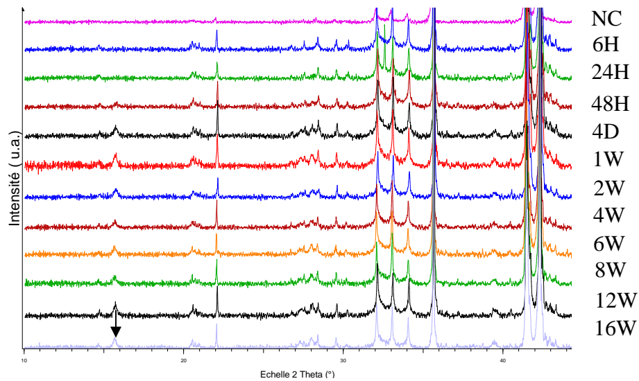
Figure S1: a. \text{La}_2\text{Ni}_7 and b. \text{La}_{1.5}\text{Mg}_{0.5}\text{Ni}_7 diffractograms after various immersion times in 8.7M KOH: from top to bottom : non corroded, 6 hours, 24 hours, 48 hours, 4 days, 1 week ; 2 weeks, 4 weeks, 6 weeks, 8 weeks, 12 weeks, 16 weeks. The black arrow corresponds to the (100) diffraction peak of the \text{La}(\text{OH})_3 phase (PDF n° 00-036-1481 ; NC = non corroded, H = hour(s), D = day(s), W = week(s))
