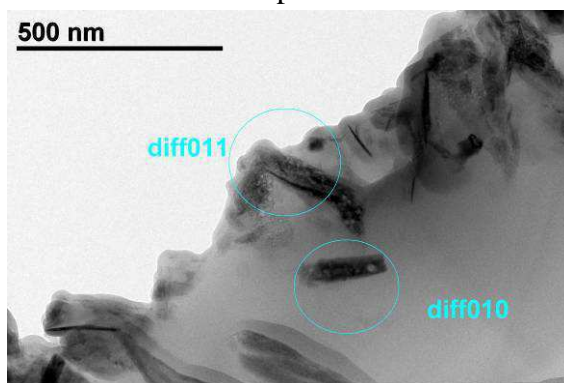
Figure S5: TEM bright field micrograph and electronic diffraction scanning area on \text{La}_2\text{Ni}_7 sample corroded 48h on 8.7M KOH
