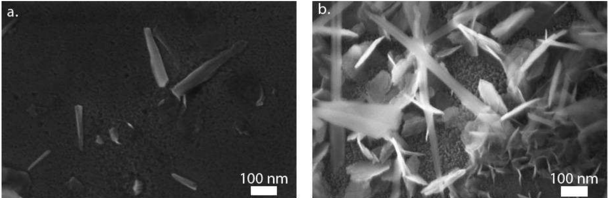
Figure 6: SEM micrographs, in InLens mode, of the metal/corrosion products interface for a. La 2 Ni 7 corroded for 6h in 8.7M KOH and b. La 1.5 Mg 0.5 Ni 7 corroded for 24h in 8.7M KOH.
