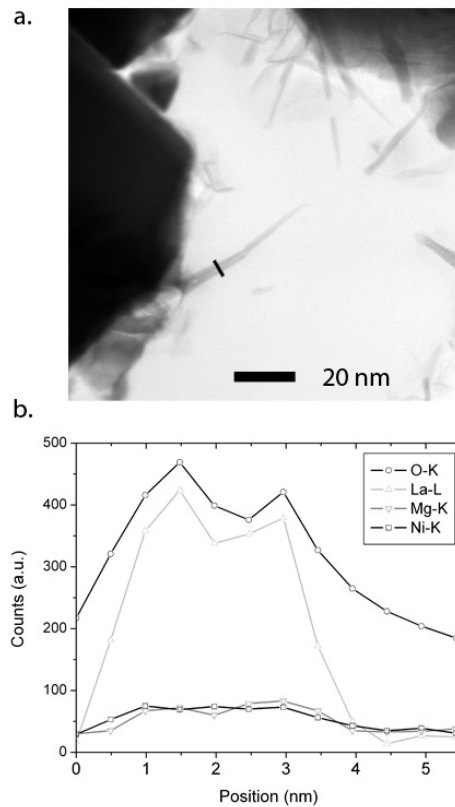
Figure 9: STEM micrograph and STEM-EDS elemental profile for the \text{La}_2\text{Mg}_{0.5}\text{Ni}_7 sample corroded 6h in 8.7M KOH.
