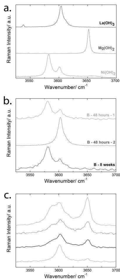
Figure 3: Micro-RS spectra recorded on a. La(OH) 3 , Ni(OH) 2 and Mg(OH) 2 references; b. La 2 Ni 7 corroded for 48 hours (2 points) and 8 weeks; c. La 1.5 Mg 0.5 Ni 7 corroded for 48 hours (4 points). Acquisition conditions 600 s.
