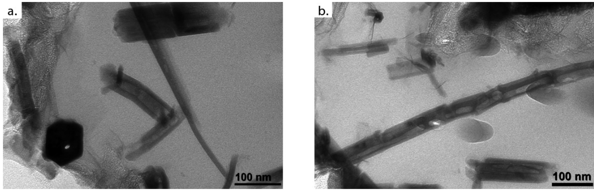
Figure 10: TEM micrograph showing the tubular structure on \text{La}_2\text{Mg}_{0.5}\text{Ni}_7 sample corroded 8 weeks in 8.7M KOH.
