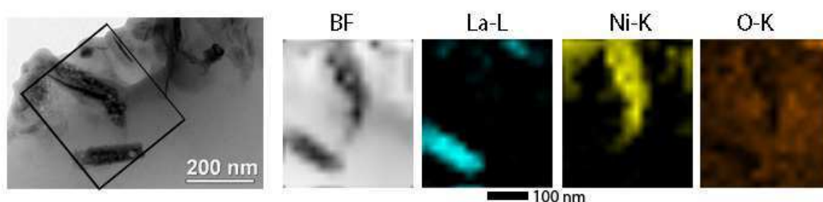
Figure 7: TEM micrograph and EDS-STEM elemental mapping of La, Ni and O for the \text{La}_2\text{Ni}_7 sample corroded 48h in 8.7M KOH solution.
