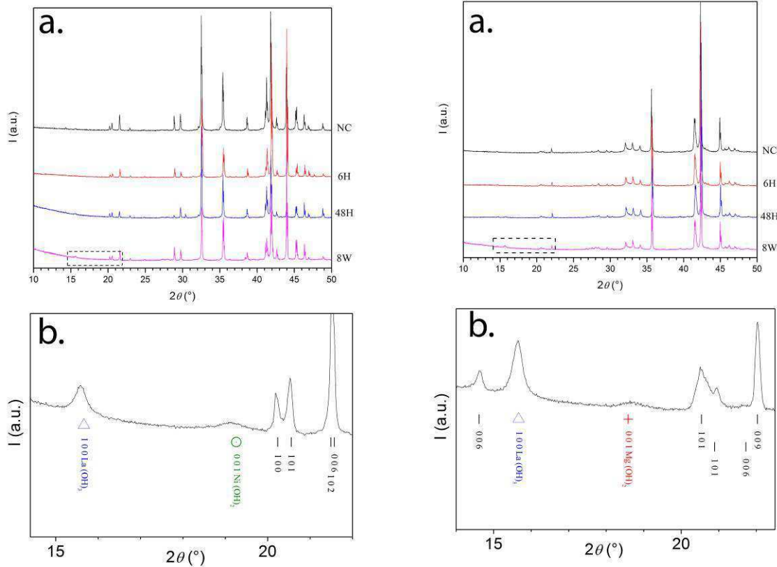
Figure 1: La 2 Ni 7 diffractograms after various immersion times in 8.7M KOH; a. from top to bottom: non corroded (NC), 6 hours (6H), 48 hours (48H) and 8 weeks (8W); b. low theta region shown in the dashed rectangle, with longer acquisition time for the sample soaked 8 weeks in 8.7M KOH. The (100) diffraction peak of La(OH) 3 (triangle; PDF n°00-036-1481) and the (001) diffraction peak of Ni(OH) 2 (circle; PDF n°04-012-5845) are shown beside the peaks of the main phase (vertical bars; Ce 2 Ni 7 -type).
