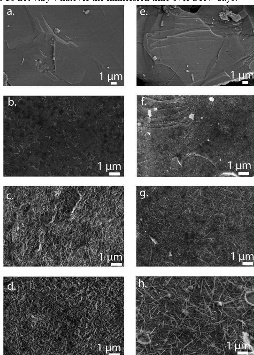
Figure 4: SEM micrographs at magnification 10k, in SE2 mode, of (a.) non corroded \text{La}_2\text{Ni}_7 sample and \text{La}_2\text{Ni}_7 sample corroded for (b.) 6h, (c.) 48h and (d.) 8 weeks; (e.) non corroded \text{La}_{1.5}\text{Mg}_{0.5}\text{Ni}_7 sample and \text{La}_{1.5}\text{Mg}_{0.5}\text{Ni}_7 sample corroded for (f.) 6h, (g.) 48h and (h.) 8 weeks.
