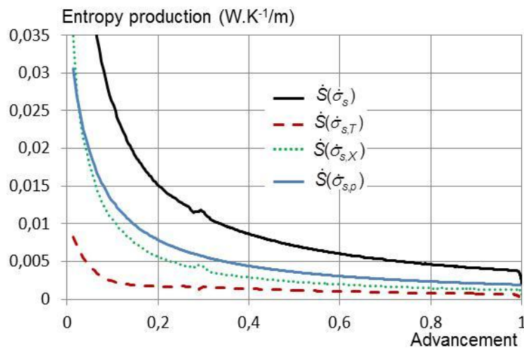
Figure 8: Entropy productions related to kinetics, mass and heat transfer, and total entropy production occurring in a reactive layer of an open system. Results are given per meter of reactor depth ( W \cdot K^{-1}/m ).
