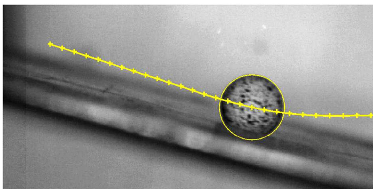
Fig. 15 Measured positions (+) and position of the ball (circle) at t=0.65\text{ms} during the contact with the specimen.
