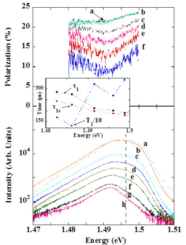
FIG. 8. Energy-dependent TRPL at 10 K. The bottom panel shows the luminescence spectra at 10 K taken after a delay of 50 ps, corresponding to the maximum of the signal (a), 150 ps (b), 400 ps (c), 550 ps (d), 700 ps (e), 900 ps (f), 1300 ps (g), and 2000 ps (h) after the laser pulse. The top panel shows the corresponding light polarization spectra, where curves g and h have been omitted, as well as regions of poor signal-to-noise in the polarization spectra. The inset shows the energy dependences of \tau_1 , and \tau_{1s} , extracted from the sum and difference transients according to Eq. (7) and of the resulting spin relaxation time T_1 .
