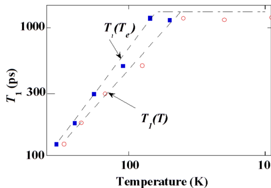
FIG. 7. Dependence of the spin relaxation time T_1 as a function of the lattice temperature T and of the temperature of the photoelectron gas T_e . At high temperature, these dependences follow a power law, of exponents 1.16 and of 1.41, respectively. The latter exponent is close to the one predicted by the Bir Aronov Pikus model for relaxation by exchange with holes.
