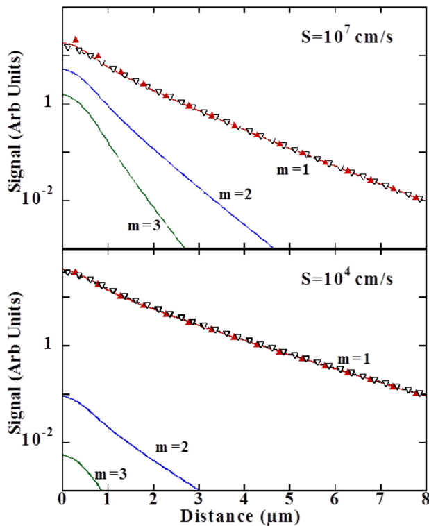
FIG. 9. The solid lines show the concentration profiles corresponding to the first 3 spatial modes, calculated using Eq. (8) for D=100 \text{ cm}^2/\text{s} , \tau=300 \text{ ps} , \sigma=0.5 \mu\text{m} , \alpha_l=0 , and S'=0 . S is taken equal to 10^4 cm/s in the bottom panel and 10^7 cm/s in the top panel. The sums of these modes are shown by full triangles and are in good agreement with the profiles, shown by open triangles, calculated using Eq. (A8) and using S=S'=0 and L=L_1 . The effect of modes of m > 1 is negligible for S=10^4 cm/s, and only slightly affects the profile for S=10^7 cm/s for r < 1 \mu\text{m} .
