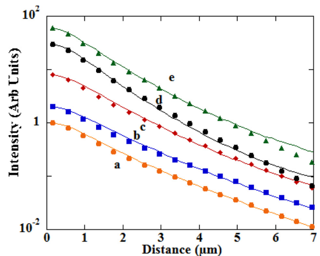
FIG. 6. Temperature effects investigated using \mu PL. Experimental spatial decay of the luminescence intensity as a function of distance to the laser excitation spot, for selected lattice temperatures of 300 K (a), 80 K (b), 40 K (c), 15 K (d), and 8 K (e). The curves, normalized at the maximum, were shifted upwards for clarity. Also shown by dots are curves calculated using Eq. (A8), using an effective diffusion length given in Table I.
