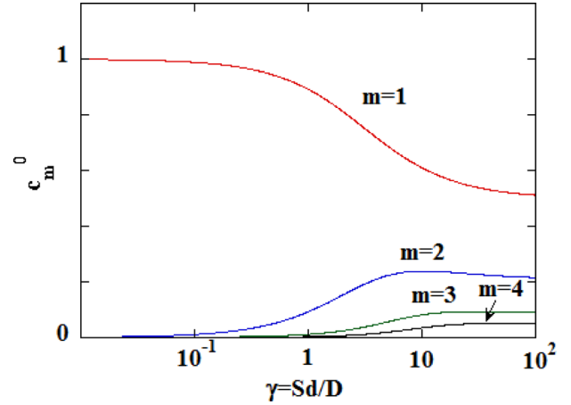
FIG. 3. Dependence of the amplitudes c_m^0 of the various modes defined in Eq. (7), calculated using Eq. (A4) and using in Eq. (1) \alpha_l = 0 . For a passivated surface ( \gamma = 0 ), only one mode is present in the transient, of time equal to \tau .
