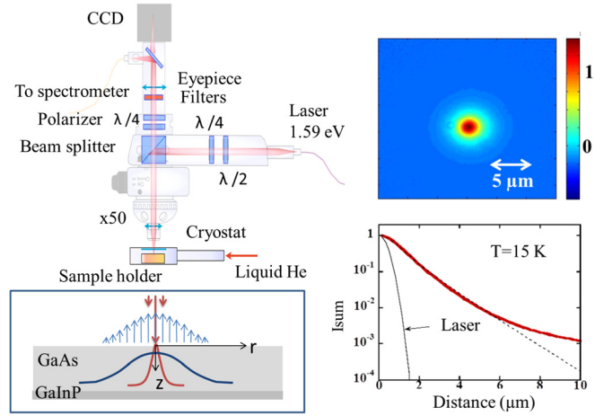
FIG. 2. Microphotoluminescence. The left panel shows the principle of the \mu PL technique, in which a laser is tightly focused onto the sample, and where an image (shown in the top right panel) is taken using a CCD camera. The bottom right panel shows an angular-integrated section of this image in the same conditions as Fig. 1, together with a fit and the cross section of the laser profile.
