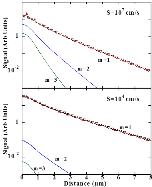
FIG. 9. The solid lines show the concentration profiles corresponding to the first 3 spatial modes, calculated using Eq. (8) for D=100\text{ cm}^2/\text{s} , \tau=300\text{ ps} , \sigma=0.5\text{ }\mu\text{m} , \alpha_f=0 , and S'=0 . S is taken equal to 10^4 cm/s in the bottom panel and 10^7 cm/s in the top panel. The sums of these modes are shown by full triangles and are in good agreement with the profiles, shown by open triangles, calculated using Eq. (A8) and using S=S'=0 and L=L_1 . The effect of modes of m>1 is negligible for S=10^4 cm/s, and only slightly affects the profile for S=10^7 cm/s for r<1\text{ }\mu\text{m} .
