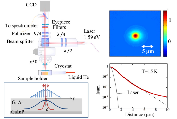
FIG. 2. Microphotoluminescence. The left panel shows the principle of the \mu PL technique, in which a laser is tightly focused onto the sample, and where an image (shown in the top right panel) is taken using a CCD camera. The bottom right panel shows an angular-integrated section of this image in the same conditions as Fig. 1, together with a fit and the cross section of the laser profile.
