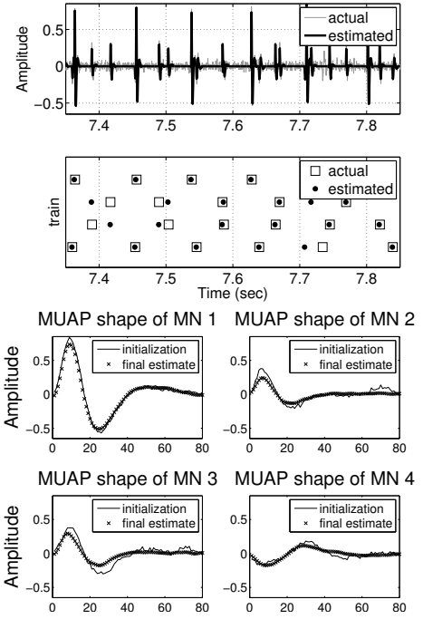
Figure 6. Reconstruction without noise of the signal for four identified spike trains of an iEMG signals: the reconstruction with the expert and estimated spike trains, and the estimated impulse responses (experimental signal)
