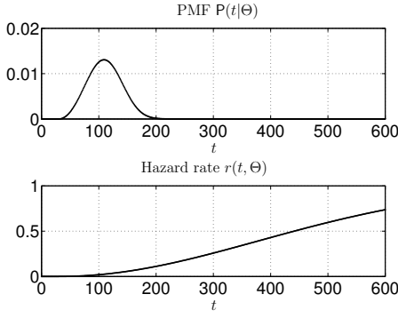
Figure 2. Weibull PMF and hazard rate ( t_0 = 120 , \beta = 3 , t_R = 30 )
