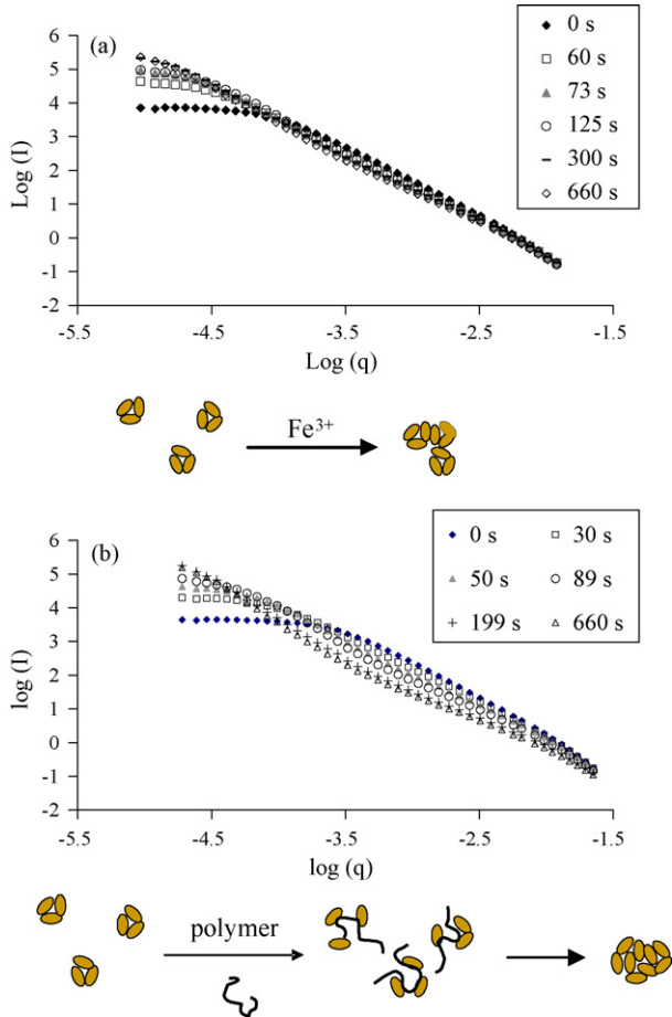
Fig. 7. Variation of \log(l) versus \log(q) during coagulation in Jar-test: (a) FeCl 3 and (b) C595 at 0.15 ppm.
