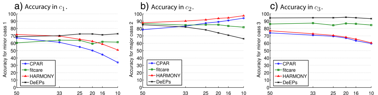
Fig. 8. Per-class accuracy results when the classes c_1 and c_3 are reduced to 50, 33, 25, 20, 16, and 10% of their original sizes.
