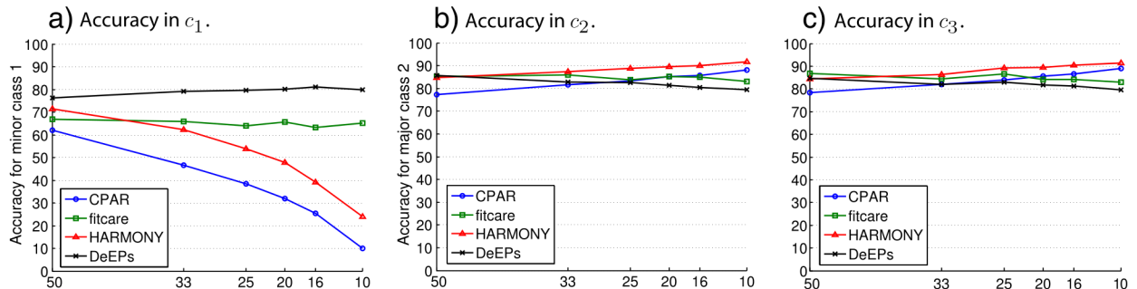
Fig. 6. Per-class accuracy results when the class c_1 is reduced to 50, 33, 25, 20, 16 and 10% of its original size.
