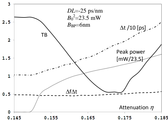
Fig. 6. Properties of mode-locked pulse at different cavity attenuation \eta . Pulse's width is divided by 10, its peak power is normalized to B_0^2=23.5 mW.
