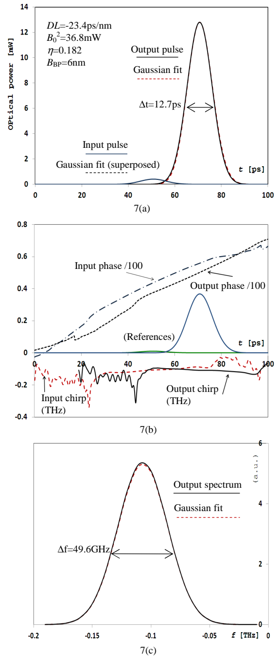
Fig. 7. Pulses obtained with DL=-23.4 , B_0^2=36.8 mW and \eta=0.182 . 7(a): Input and output pulses' shapes and their Gaussian fits; 7(b): Correspondent optical phases (/100) in radian and chirps in THz; 7(c): Output spectrum with a Gaussian fit.
