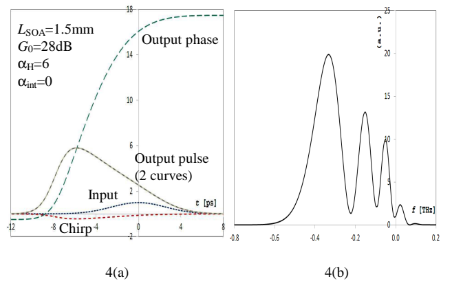
Fig. 4. Amplification of a 3ps Gaussian pulse by SOA. 4(a): The input and the output pulses' (theory and calculation) intensities in a linear scale, output pulse's phase in radian, and its chirp in THz. Notice that t is traced in a moving coordinate at the group velocity. 4(b): Spectrum of the output pulse.
