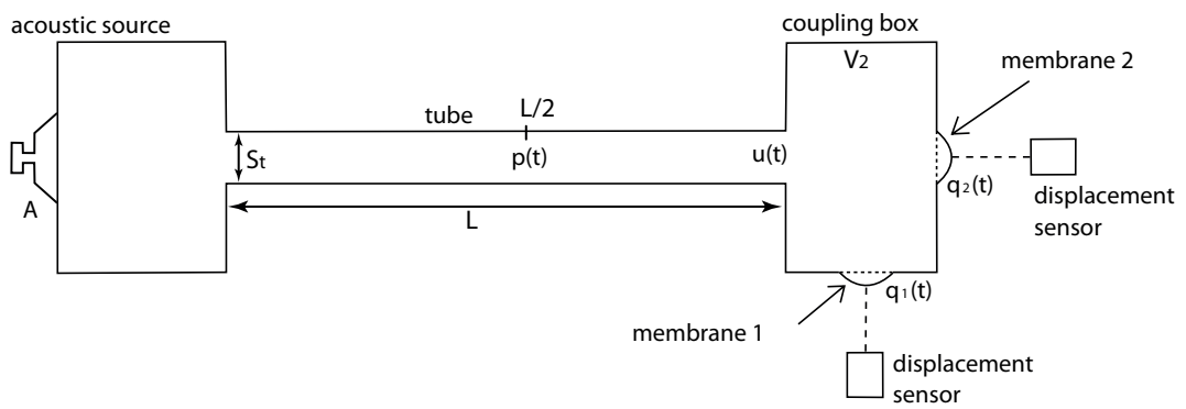
Figure 2: Scheme of the experimental set-up with two membrane absorbers. A : amplitude voltage of the sinusoidal input signal. p(t) : acoustic pressure at the middle of the tube. u(t) : air displacement at the end of the tube. q_1(t) and q_2(t) : respective displacements of the centers of the membranes 1 and 2.
