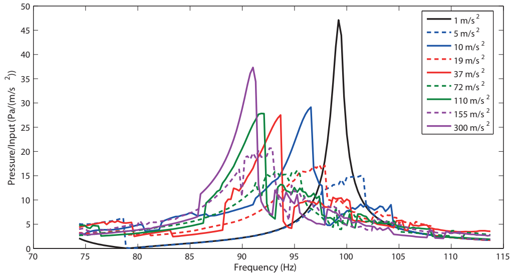
Figure 7: Numerical results. Frequency responses with four different membranes for nine different input levels.
