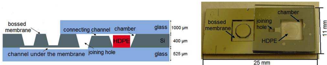
Fig. 2: The MEMS high doses radiation sensor: (a) cross-sectional view; (b) sensor at a glance. Anodic bonding in air, 450°C, 600 V
