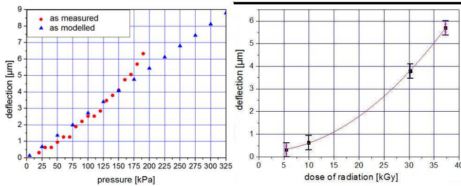
Fig. 4: Sensor response for (5×5×0.08 mm 3 ) membrane: (a) deflection as a function of pressure inside the chamber; (b) deflection as a function of radiation dose.
