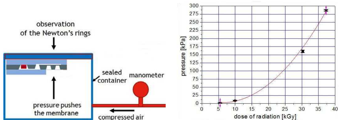
Fig. 5: Differential method for measurement of pressure inside the sensor after irradiation: (a) scheme of the measurement set-up; (b) pressure inside the sensor as a function of dose of radiation.
