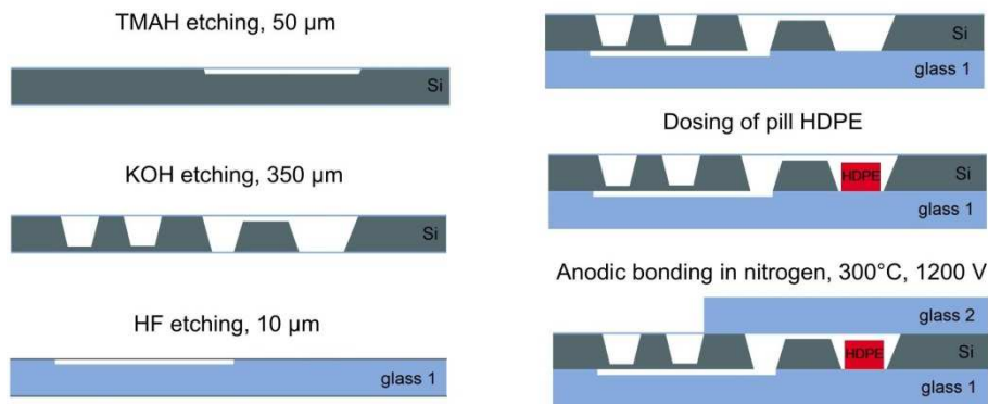
Fig. 3: The fabrication of the sensor – main technological steps.
