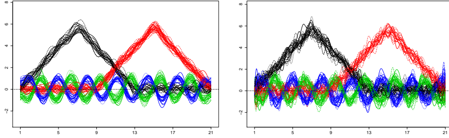
FIG 4.4. Simulated curves with cubic spline smoothing (left) and Fourier basis smoothing (right).
