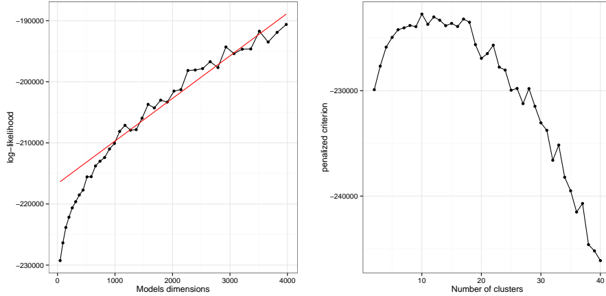
FIG 4.2. Model selection plots for Paris: log-likelihood with respect to model dimensionality and its estimated linear part (left), slope heuristic criterion with respect to K (right).
