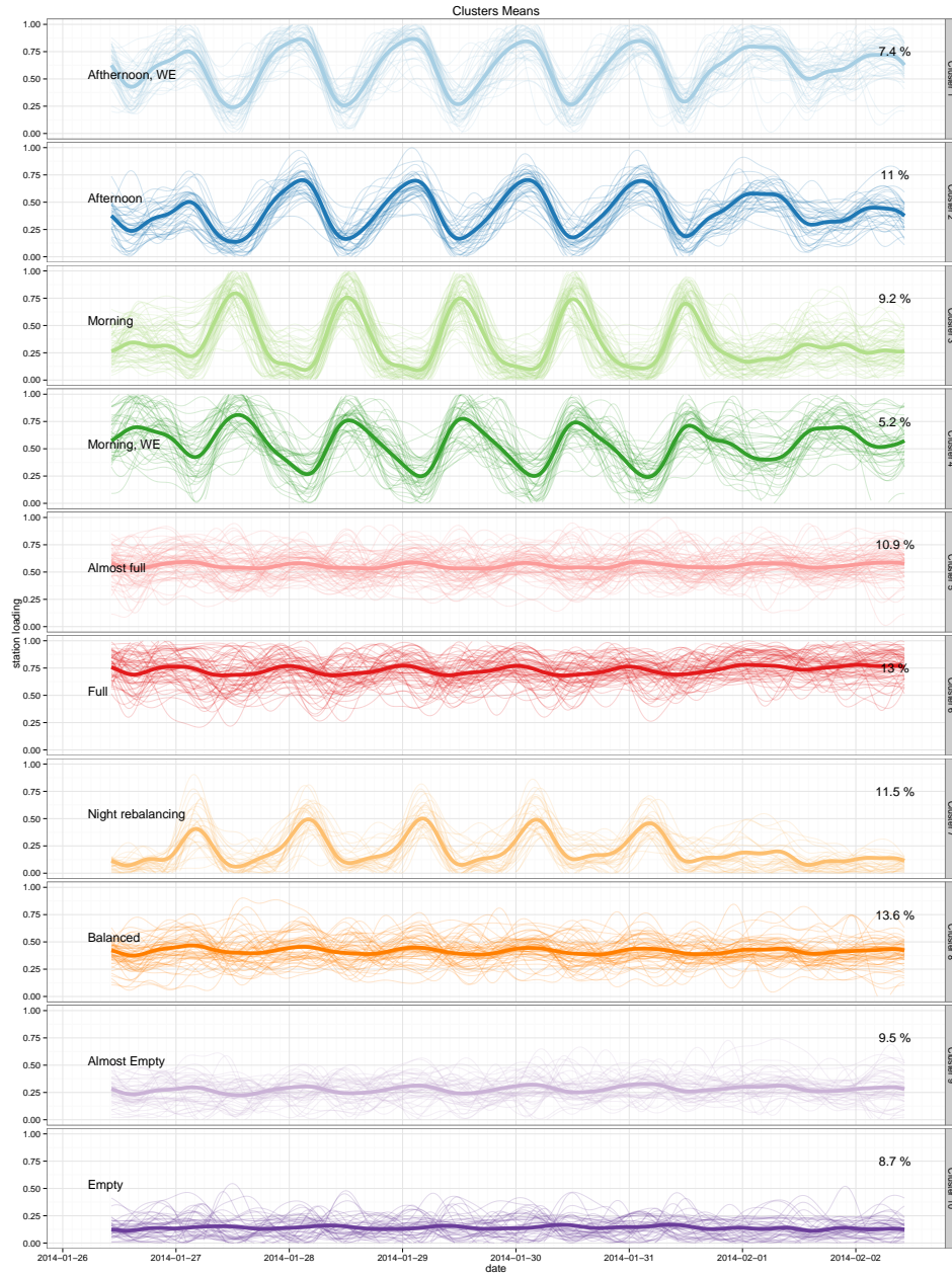
FIG A.1. Cluster mean profiles together with 1000 randomly sampled curves for the whole data set (Paris, London, Bruxelles, Lyon, Seville and Nantes).
