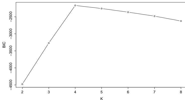
FIG 3.2. Selection of the number of clusters using BIC on the simulated data (actual value of K is 4).
