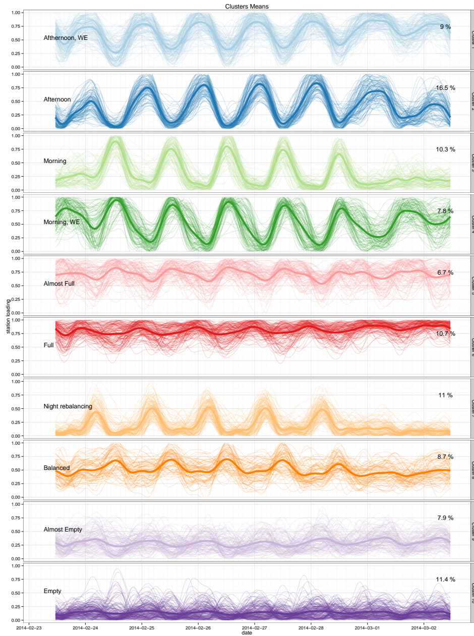
FIG 4.3. Cluster mean profiles together with 1000 randomly sampled curves. The name of the clusters and their proportions are also provided.
