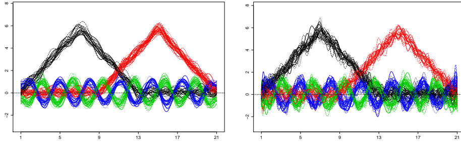
FIG 3.4. Simulated curves with cubic spline smoothing (left) and Fourier basis smoothing (right).
