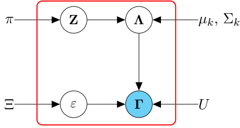
FIG 2.1. Graphical representation for the model \text{DFM}_{[\Sigma_k, \beta]} .
