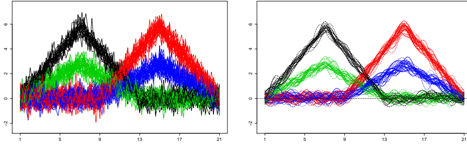
FIG 3.1. Raw and smoothed simulated curves.
