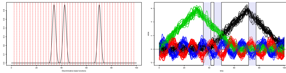
FIG 3.6. Discriminative functions among the Spline basis functions: selected basis functions (left) and original data with, highlighted in grey, the time periods associated with the selected basis functions (right).
