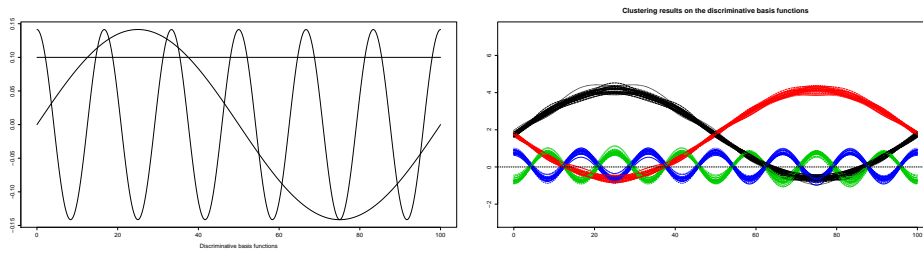
FIG 3.5. Discriminative functions among the Fourier basis functions: selected basis functions (left) and data projected on the selected basis functions (right).
