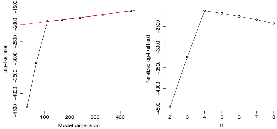
FIG 3.3. Selection of the number of clusters using the slope heuristic on the simulated data (actual value of K is 4).
