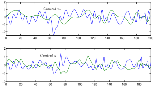
Figure 6. Control inputs u_r(k) and u(k)
