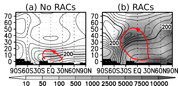
Figure 2. Zonal mean temperature (contoured with an interval of 10 K) and cloud ice mole mixing ratio (shaded, ppm) during northern summer ( L_s = 60-90^\circ ) for simulations (a) x_{35}^* and (b) x_{35} . The 5 \times 10^9 \text{ kg s}^{-1} contour of the stream function is also represented in red. Y axis is altitude in kilometers.
