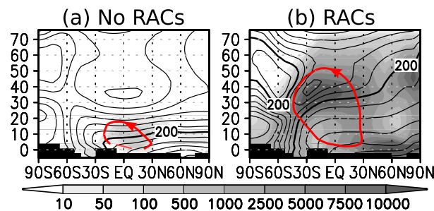
Figure 2. Zonal mean temperature (contoured with an interval of 10 K) and cloud ice mole mixing ratio (shaded, ppm) during northern summer ( L_s = 60\text{--}90^\circ ) for simulations (a) x_{35}^* and (b) x_{35} . The 5 \times 10^9 \text{ kg s}^{-1} contour of the stream function is also represented in red. Y axis is altitude in kilometers.
