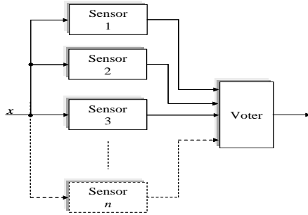
Fig.5 Hardware redundancy
