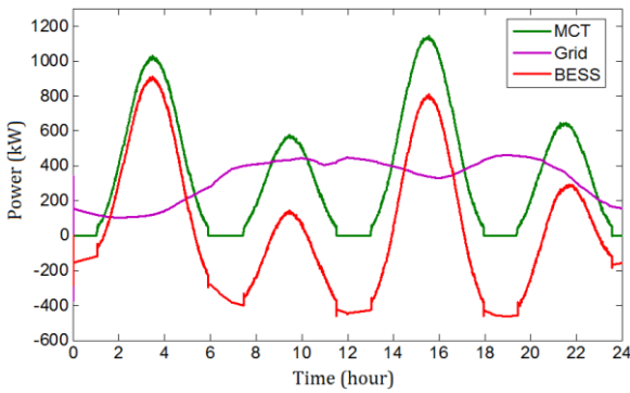
Fig. 9. Powers of the MCT system with BESS during one day.
