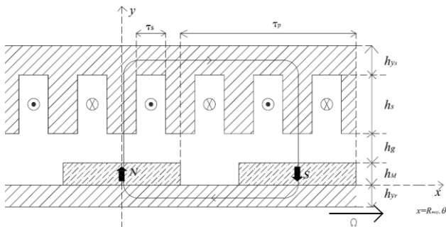
Fig. 3. AFPM generator geometry.
