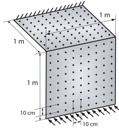
Figure 3. Simulated experimental structure consisting of two plates connected by a joint
