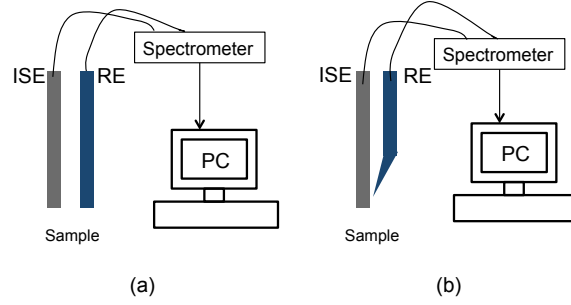
Figure 4: Techniques scheme based on ISE method (a) Normal RE and (b) RE with Luggin capillary
