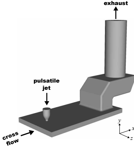
FIG. 8. Computational domain.
