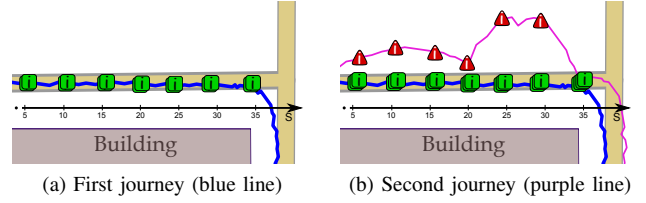
Fig. 4: A correct map area close to a large building. Red triangles (resp. green squares) are for estimates which the method has isolated as faulty (resp. true).
