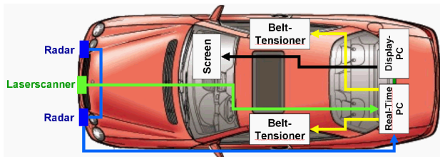
Fig. 1. Hardware architecture of the experimental vehicle showing sensors, actuators, computers and interconnects.
