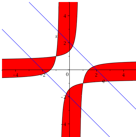
Figure 1: The set S := \{(q, s) : K(q, s) < 0\} \setminus \{(q, s) : q = 2 - s \text{ or } q = -2 - s\} is given by the red (dark) area without the diagonal blue (dark) lines.
