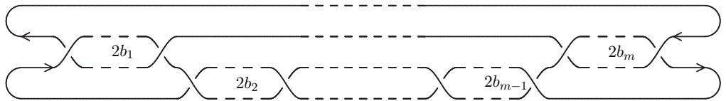
Figure 2: Oriented two-bridge links ( m odd)
