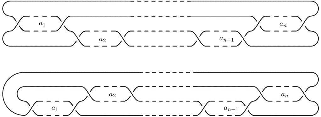
Figure 1: Conway's normal forms ( n odd or even)
