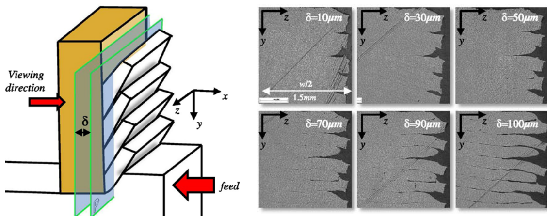
Fig. 8 Successive cuts of the chip through thickness showing an open crack at the left end but connected material within the hydrostatic stress zone
