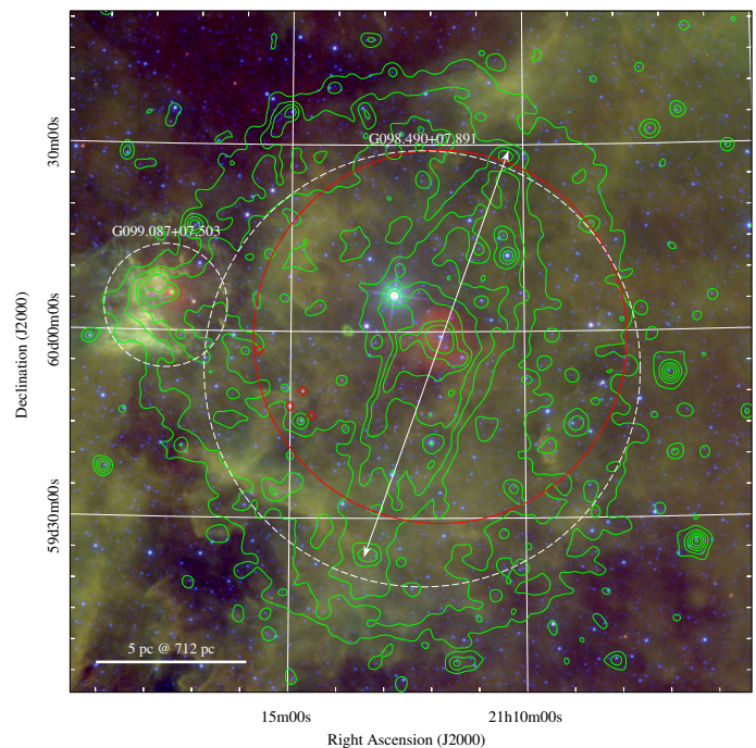
Fig. 2. Mid-infrared image of Sh 2-129 obtained from the WISE All-Sky Atlas. The blue, green, and red colours code to the WISE infrared bands W2 , W3 , and W4 centred at 4.6, 12, and 22 \mu\text{m} -filters, respectively. The green contour map is the same [O III] image shown in Fig. 1. The dashed white circles indicates the two (radio quiet) H II regions in the WISE catalog of Galactic H II regions (Anderson et al. 2014). The red diamonds mark the classical T Tauri star candidates that we have identified inside the 30' -radius red circle centered on HR 8119 (see labels in Fig. 3).
