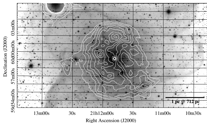
Fig. 11. [O III] emission from the central part of Ou4 vs. 22 \mu\text{m} emission. The color scale of the [O III] image is logarithmic. The contour map is the 22 \mu\text{m} emission of the W4-filter image from 89.375 to 92.5 digital numbers (DN) with linear step of 0.446 DN (i.e., from 2.471 to 2.557 mJy/arcsec 2 with linear step of 0.012 mJy/arcsec 2 ). The linear scale is shown in the bottom-right corner.
