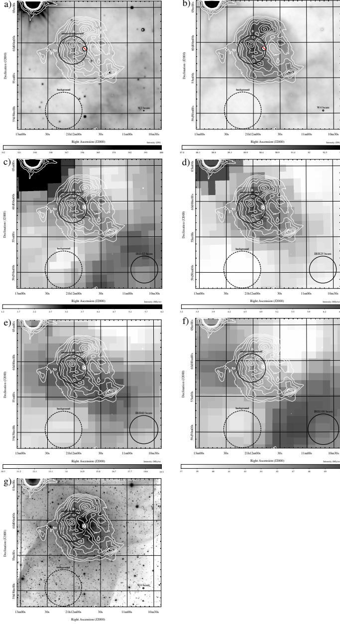
Fig. 13. Mid- to far-infrared views of the central part of Ou4. a) WISE 12- \mu m (W3-filter) image. b) WISE 22- \mu m (W4-filter) image. c) IRIS 12- \mu m image. d) IRIS 25- \mu m image. e) IRIS 60- \mu m image. f) IRIS 100- \mu m image. g) INT [O III] image for comparison purpose. The contour map is the 22 \mu m emission from 89.375 to 92.5 digital numbers (DN) with linear step of 0.446 DN (i.e., from 2.471 to 2.557 mJy/arcsec 2 with linear step of 0.012 mJy/arcsec 2 ). The FWHM resolution is plot in the bottom-right corner of each panel. The two large circles are the regions used for the aperture photometry (see text and Fig. 14).
