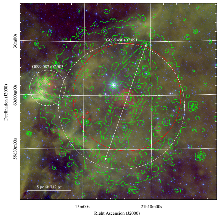
Fig. 2. Mid-infrared image of Sh 2-129 obtained from the WISE All-Sky Atlas. The blue, green, and red colours code to the WISE infrared bands W2, W3, and W4 centred at 4.6, 12, and 22\ \mu\text{m} -filters, respectively. The green contour map is the same [O III] image shown in Fig. 1. The dashed white circles indicate the two (radio quiet) H II regions in the WISE catalog of Galactic H II regions (Anderson et al. 2014). The red diamonds mark the classical T Tauri star candidates that we have identified inside the 30' -radius red circle centered on HR 8119 (see labels in Fig. 3).
