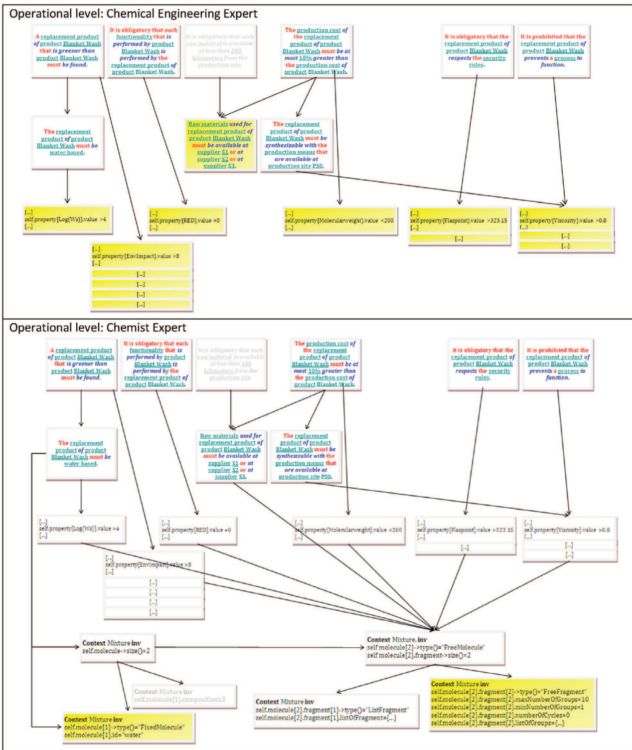
Fig. 10. Operational level construction Illustration of the sequential construction of the requirements tree for ink blanket-wash product.
