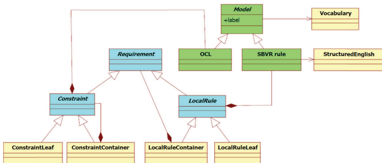
Fig. 4. An UML2 model of requirement.
