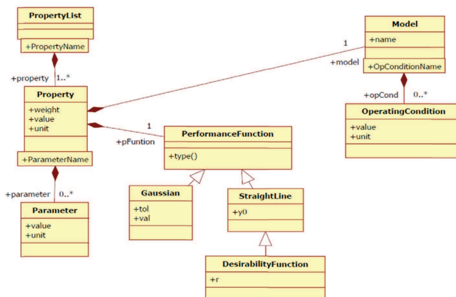
Fig. 5. Class diagram used for the OCL description of the constraints on the properties.
