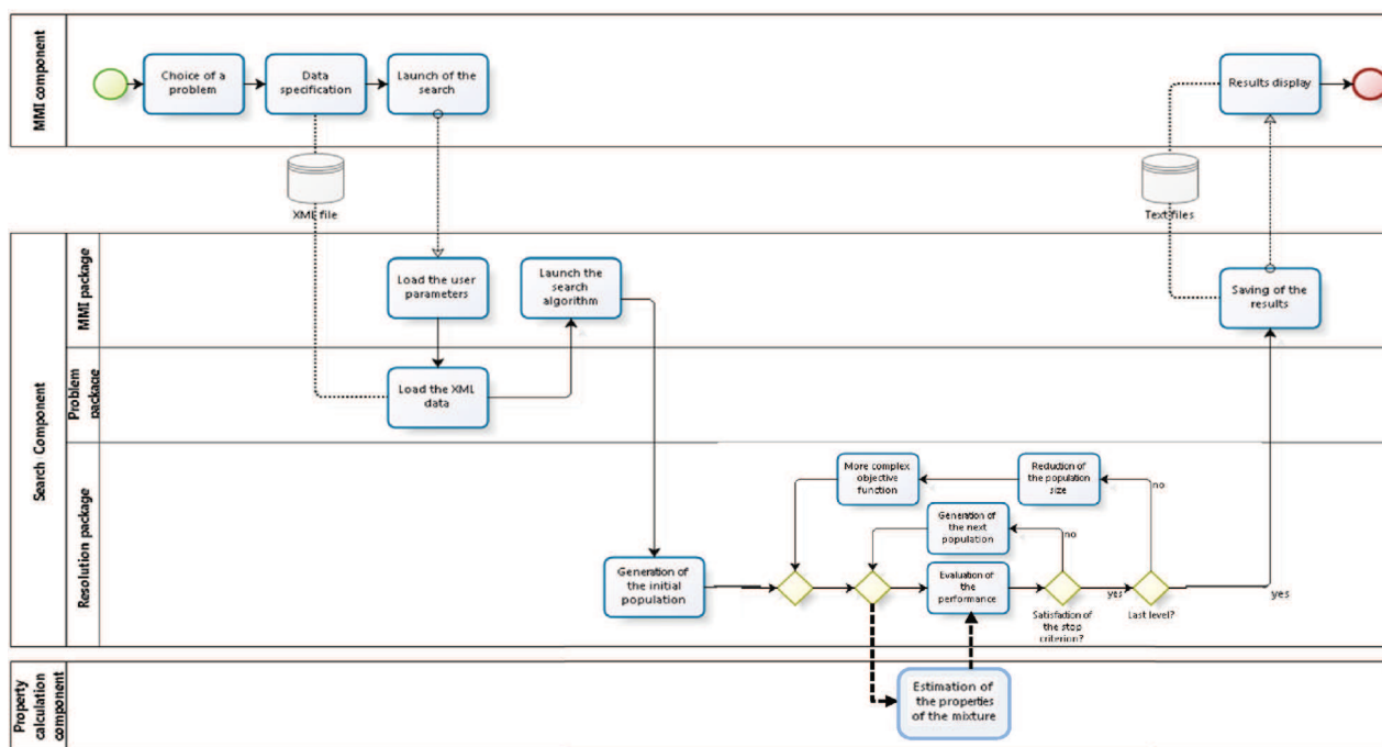
Fig. 7. BPMN diagram of the three IBSS components behavior.
