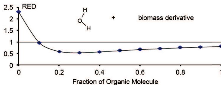
Fig. 11. Performance and property values for the best biomass derivative mixture and influence of its fraction on its ability to dissolve the ink (RED property).
