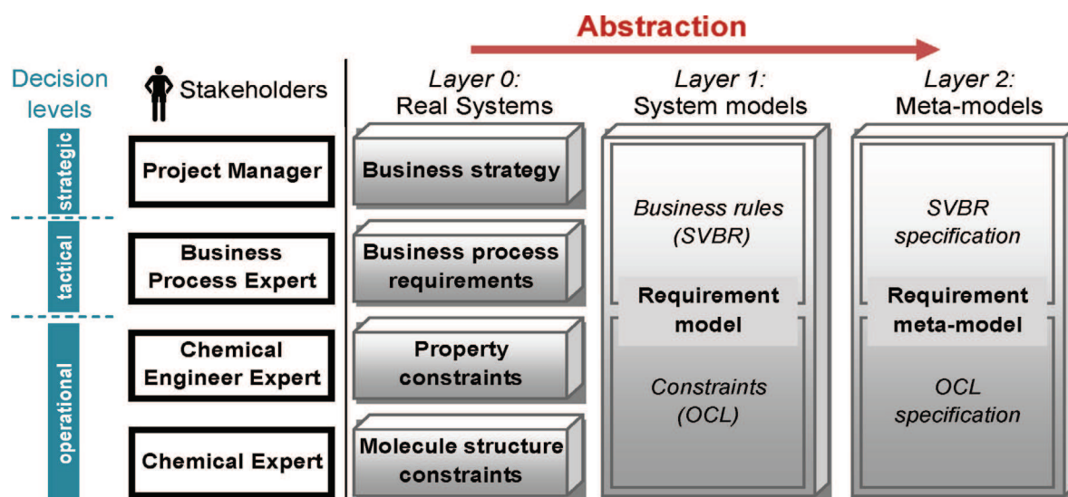
Fig. 3. A simplified multi-level and multi-layer approach for the product design Intelligence phase.
