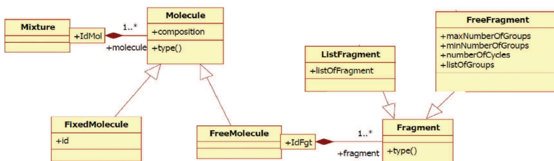
Fig. 6. Class diagram used for the OCL description of the constraints on the molecular structures.
