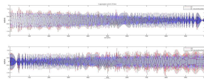
FIGURE 9: reconstruction of each source in time
