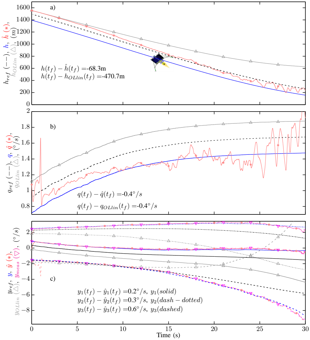
Fig. 4. Evolution of \hat{h} , \hat{q} and the outputs of the observer \hat{Y} = [\hat{y}_1, \hat{y}_2, \hat{y}_3]^T in the nonlinear system equipped with an LPV observer. One can see from this figure that the estimated states gave good raw estimates of the actual states despite the intrinsic sensitivity of the system to noise during the last few seconds. The estimated outputs were very close to the actual outputs of the nonlinear system. The estimated states were initialized in such a way that \Delta\hat{h}_0 = 60\text{m} , \Delta\hat{q}_0 = -0.2^{\circ}/\text{s} . The open loop linearized system states correspond to a simulation where the linearized system is run in open loop from the same initial conditions as the observer (states are denoted h_{OLLin} , q_{OLLin} and y_{OLLin} ).
