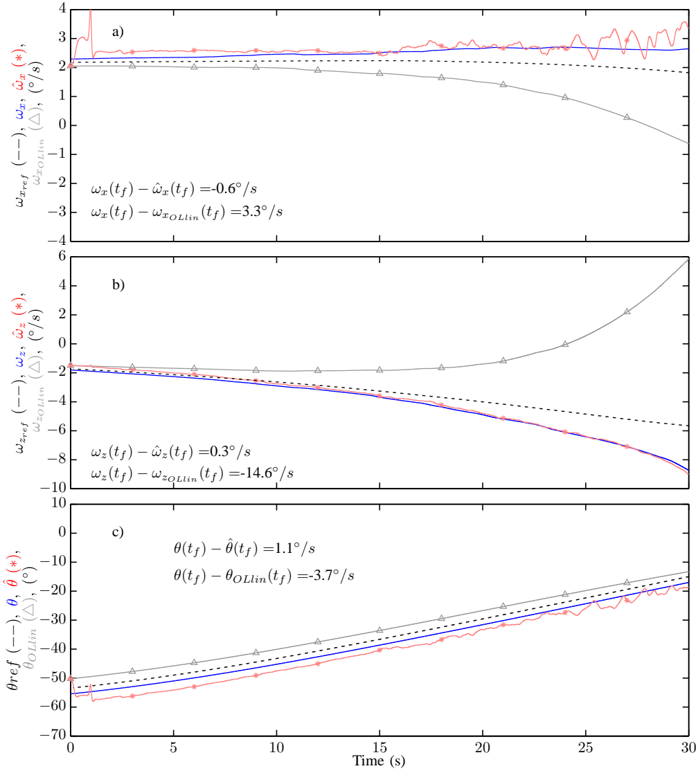
Fig. 3. Evolution of estimated \hat{\omega}_x , \hat{\omega}_z and \hat{\theta} in the nonlinear system with the newly designed LPV observer. The three sub-figures show the actual state of the nonlinear system (blue line), the reference state (dashed black line), the open loop linearized system ( \Delta -mark line) and the estimated states (*-mark line). The open loop linearized system states correspond to a simulation where the linearized system is run in open loop from the same initial conditions as the observer (states are denoted \omega_{x_{OLlin}} , \omega_{z_{OLlin}} and \theta_{OLlin} ). One can see that the estimated states converged quickly toward the actual states of the nonlinear system, which were deliberately intended not to follow the reference trajectory. It should be noted in addition that the open loop linearized system alone would not have sufficed to obtain an accurate state estimation. Estimated states were initialized, giving \Delta\hat{\omega}_{x_0} = -0.126^\circ/s , \Delta\hat{\omega}_{z_0} = 0.23^\circ/s , \Delta\hat{\theta}_0 = 3.23^\circ .
