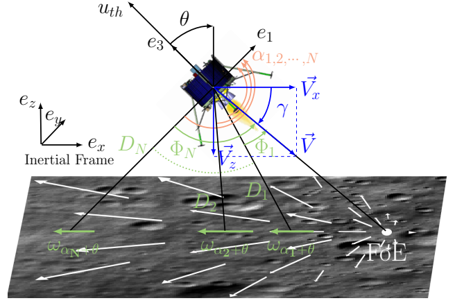
Fig. 1. Definition of the body-fixed frame \mathcal{B} , the inertial frame \mathcal{I} and notations for the lander's dynamics and the optic flow. Example of a N VMS setup. Sensors fixed to the lander's structure measured the OF \omega_{\alpha_N + \theta} depending on the lander's position, velocity, pitch angle and pitch angular velocity (see (5)). It can be noted that \Phi(t) = \alpha + \theta(t) + \gamma(t) . The canonical vector e_2 of \mathcal{B} was not included here for the sake of clarity.
