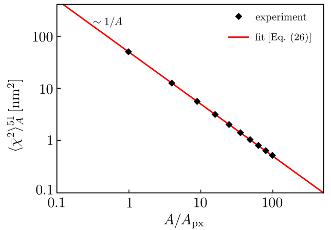
FIG. 7. The mean-square amplitude of the camera noise averaged over an area A containing N pixels of area A_{\text{px}} . The noise decreases exceptionally well with 1/A \sim 1/N , proving the camera noise is independent for different pixels.
