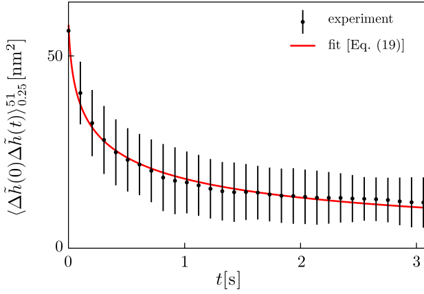
FIG. 9. Measured temporal correlation function (every second data point presented) is fitted with the expression given in Eq. (19). The fitting procedure provides \sigma = 13.0 \times 10^{-6} \text{ J/m}^2 and \gamma = 1.0 \times 10^7 \text{ J/m}^4 .
