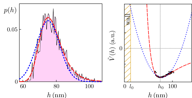
FIG. 2. Experimental height probability distribution (black line) and the respective effective potential (black symbols) are shown in the left and right panels, respectively. Fitting the data with a potential of the Mie or the harmonic form (right), and their Boltzmann factors (left), yields the red dashed and the blue dotted curves, respectively.
