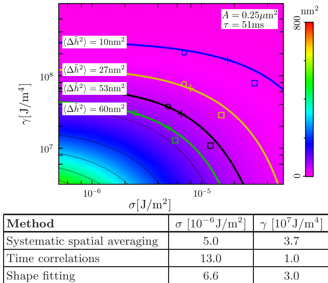
FIG. 11. A comparison of fitting procedures for a single vesicle is shown in the table and for four vesicles in the graph. The vesicle discussed in the manuscript and fittings shown in Figs. 7–10 is indicated by black lines and symbols. Circles denote results of determining the potential strength and the tension by the method of systematic averaging, while crosses and squares are obtained by fitting the shape and the time-dependent correlation function, respectively. Results of all fitting procedures for each vesicle lie very close to the appropriate contour line.
