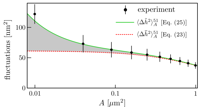
FIG. 8. Determining the tension and the potential strength by systematic spatial averaging over a square of area A . The best fit results in \sigma = 5.0 \times 10^{-6} \text{ J/m}^2 and \gamma = 3.7 \times 10^7 \text{ J/m}^4 .
