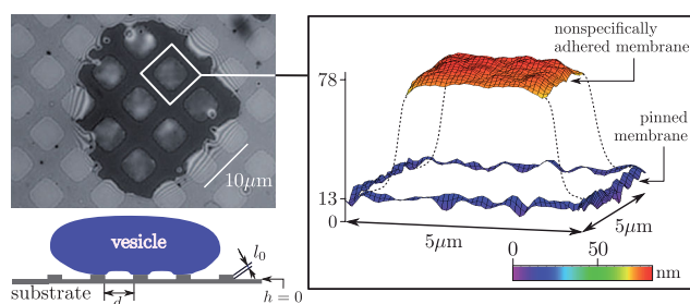
FIG. 1. RICM image of a vesicle pinned to a patterned substrate, with squares within which the membrane fluctuates in the nonspecific potential (upper-left diagram). The lower-left diagram is the schematic view. The reconstruction of the average membrane shape within one square is shown in the right panel. Only segments of a nearly planar membrane were processed to maintain accuracy in the height reconstruction [25]. The color code indicates the height above the substrate positioned at h = 0 , while l_0 denotes the thickness of the adhesive pattern on the glass substrate. The vertical axis in the right figure is in units of nanometer.
