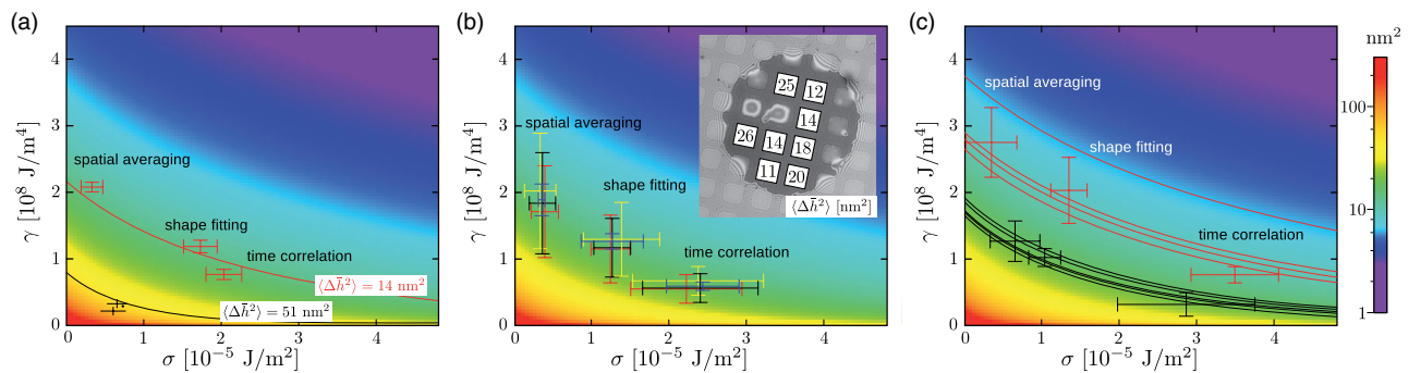
FIG. 12. Analysis of the reliability of the three approaches presented for extracting the potential strength and the tension in the membrane. The apparent fluctuation amplitude as a function of the potential strength and tension is shown as a background of each graph. The color code is given on the right. Contours associated with the apparent mean fluctuation amplitudes that are particular to each data set are displayed with solid lines. In all panels, the spatial and temporal averaging is performed with A = 0.25 \mu\text{m}^2 and \tau = 0.51 \text{ ms} , respectively. (a) Mean values and standard deviations (error bars) associated with performing the analysis on several data recordings from the same patch. Results are presented for one patch with the low (red) and one patch with the high (black) mean apparent fluctuation amplitude (indicated by numbers on the relevant contour line). (b) Mean values and standard deviations associated with averaging the fit results over the eight patches on one vesicle. The patches and the vesicle are shown in the inset by a white square. The numbers within the squares indicate the apparent mean membrane fluctuation amplitude \langle \Delta \bar{h}^2 \rangle for the particular membrane segment in units of \text{nm}^2 . The analysis was performed on two short data sequences (two subsamples shown in red and yellow) and on a long sequence (black symbols). The results of averaging over three squares with the mean apparent fluctuation amplitude between 14 and 18 \text{nm}^2 are shown in blue. (c) Mean values and standard deviations associated with averaging over fitting results from membrane patches with similar mean apparent fluctuation amplitudes on different vesicles. The results for patches with small fluctuation amplitudes, ranging from 6 to 11 \text{nm}^2 , are shown in red, while the results for large fluctuations, ranging from 18 to 20 \text{nm}^2 , are shown in black.
