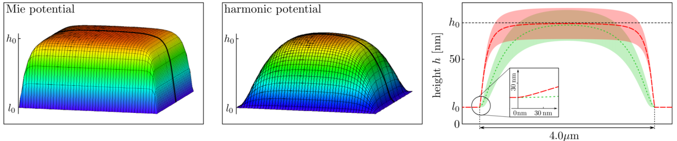
FIG. 5. Comparison of the mean membrane profile of a membrane residing in a Mie potential (left panel) and a harmonic potential of identical curvature (middle panel). The cross section through the center of the shapes is also shown, enveloped by the mean fluctuations of the shape (right panel). The profile associated with the Mie potential is shown in red, while the profile in the harmonic potential is shown in green. The inset shows a detailed view of the membrane shape near the pinning point. The shapes are determined for \sigma = 6.6 \times 10^{-6} \text{ J/m}^2 and \gamma = 3.3 \times 10^7 \text{ J/m}^4 , and h_0 - l_0 = 65 \text{ nm} , as for vesicle segments shown later in Fig. 10.
