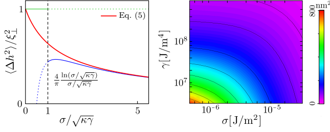
FIG. 3. Left panel: Fluctuation amplitude as a function of the membrane tension (red line). Approximations characteristic of the bending- and tension-dominated regime are shown in green and blue, respectively. Right panel: Fluctuation amplitude as a function of the tension and potential strength. Solid lines are contour lines of constant fluctuation amplitude.
