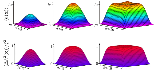
FIG. 4. Membrane in a nonspecific harmonic potential, with the minimum at the height h_0 , pinned to a square of an edge length d (in units of \xi_{\parallel} ). The universal mean membrane shape and the associated profile of the mean fluctuation amplitude (normalized by \xi_{\perp}^2 ) are shown in the top and bottom rows, respectively. All profiles are calculated for \kappa = 20 k_B T , \sigma = 0 , and \gamma = 2 \times 10^7 J/m 4 .
