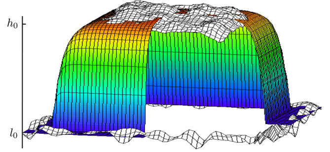
FIG. 10. Fitting the theoretically obtained mean shape (colored) to the experimentally determined mean profile of the membrane (gray). The best fit is found for \sigma = 6.6 \times 10^{-6} \text{ J/m}^2 and \gamma = 3.0 \times 10^7 \text{ J/m}^4 .
