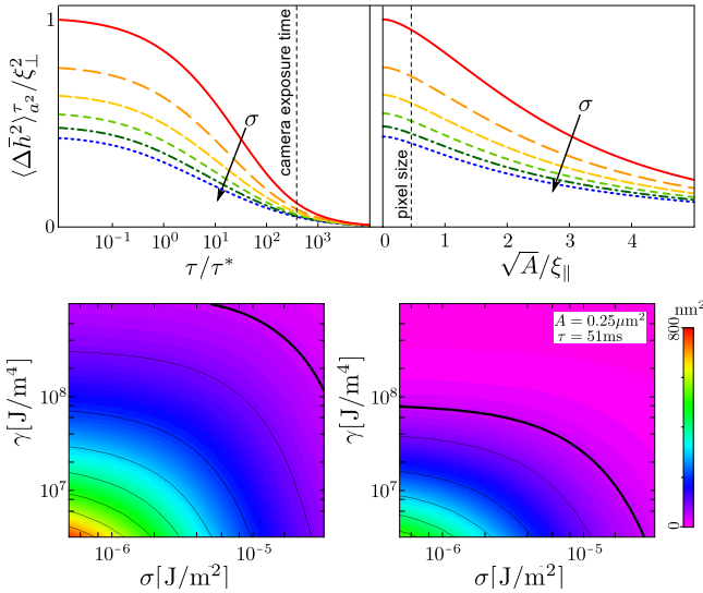
FIG. 6. Normalized apparent fluctuation amplitude as a function of temporal (upper left panel) and spatial resolution (upper right panel). The tension increases (in the direction of the arrow) from \sigma = 0 to 5\sqrt{\kappa\gamma} . The true and the apparent fluctuation amplitudes are shown in the bottom left and bottom right panels, respectively. The latter has been calculated for a fixed integration time of \tau = 51 ms and is averaged over an area of A = 0.5 \mu\text{m} \times 0.5 \mu\text{m} = 0.25 \mu\text{m}^2 . Contour lines of constant mean-square fluctuation amplitudes are indicated. Specifically, the contour lines of the true and apparent fluctuation amplitude of 50 \text{ nm}^2 are presented by the thick lines.
