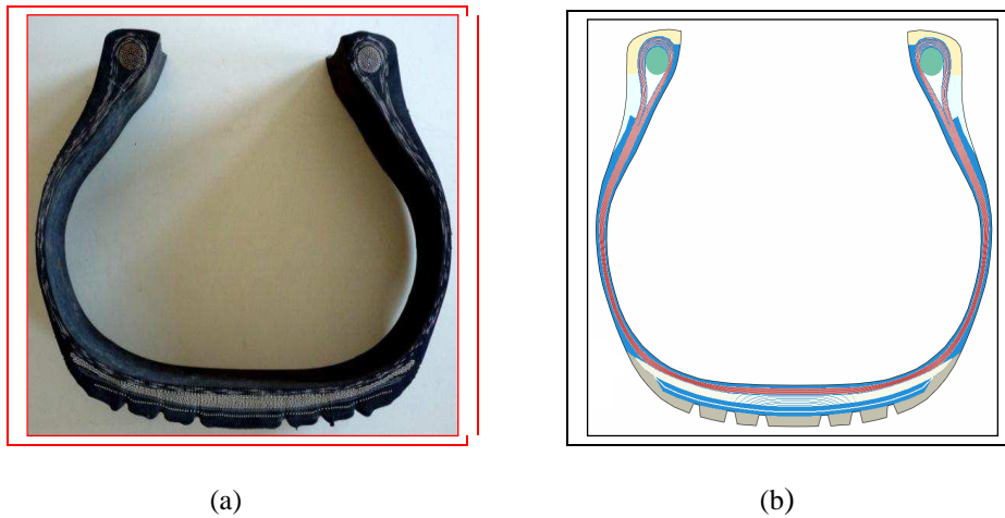
Fig.1. 2-D tire structure: (a) real cross-section of tire (b) 2-D axisymmetric FE model
