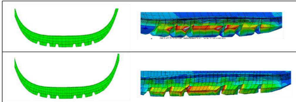
Fig.3. Comparison between old (Kongo et al. 2012) and new refined cross mesh for 2-D FEM model.
