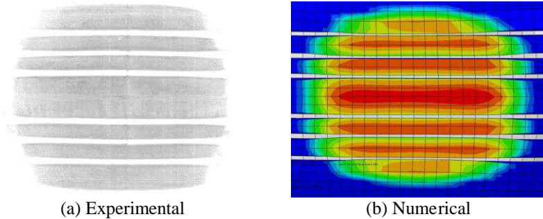
(a) Experimental (b) Numerical Fig.5. Experimental and Numerical footprints at F3 of loading
