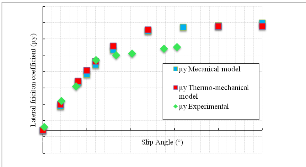
Fig. 7. Comparison between experimental data, mechanical and thermo-mechanical models Lateral friction coefficient \mu_y , under given loading conditions (vertical load, pressure and velocity)
