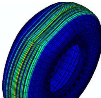
Fig.8. Temperature gradient for a cornering simulation at given velocity and slip angle
