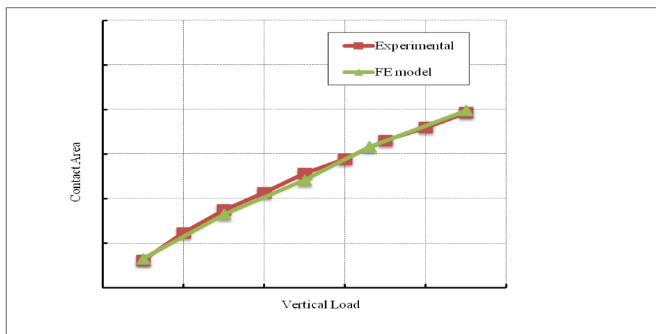
Fig.4. Evolution of contact area in the case of a grooved tire
