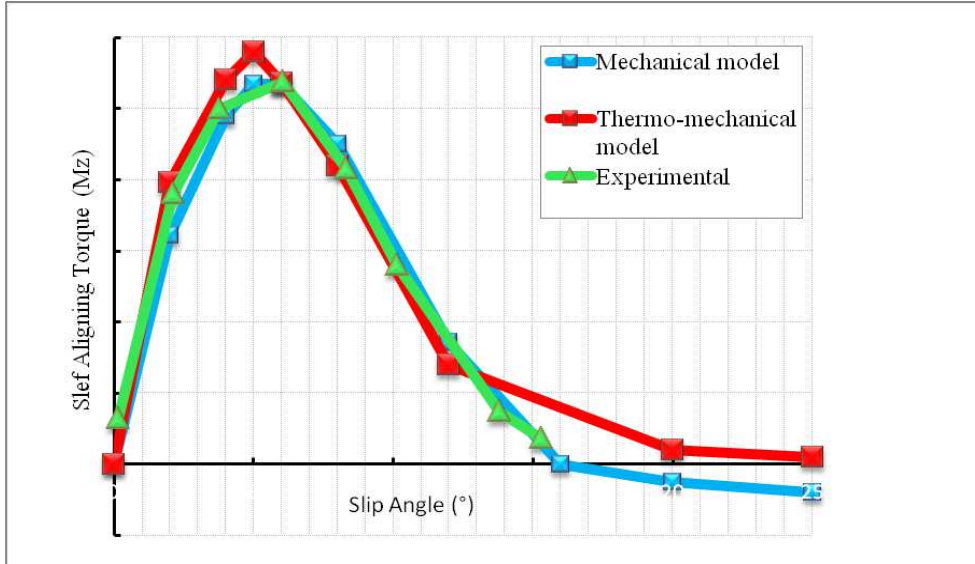
Fig. 6. Comparison between experimental data, mechanical and thermo-mechanical models Self aligning torque M_z , Under given loading conditions (vertical load, pressure and velocity)
