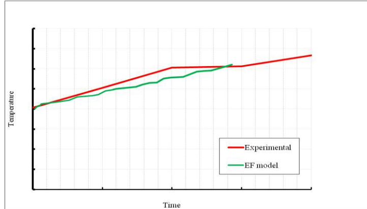
Fig.9. Temperature evolution: comparison between thermomechanical FEM and Experimental data for a cornering simulation of an aircraft tyre for given velocity and slip angle
