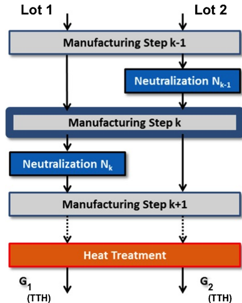
Fig. 11 Experimental principle, two different lots (1, 2) are neutralized before and after manufacturing step k . By comparing geometries of lots 1 and 2 after heat treatment, the influence of the carrier of distortion potential is revealed
