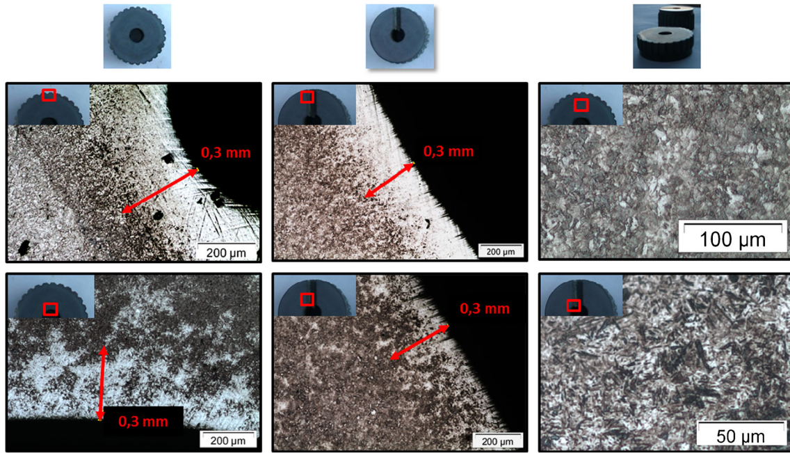
Fig. 7 Metallurgical observations after heat treatment of a lot A shaft. On the left, the first slice does not meet a radial lubrication hole. External (above) and internal (below) skins are observed. In the middle,
