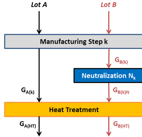
Fig. 4 Experimental principle: two different lots ( A , B ) are set up after manufacturing step k . Contrary to lot B , lot A is not neutralized. By comparing the geometry of lot A and lot B after heat treatment, the influence of the carrier of distortion potential is revealed
