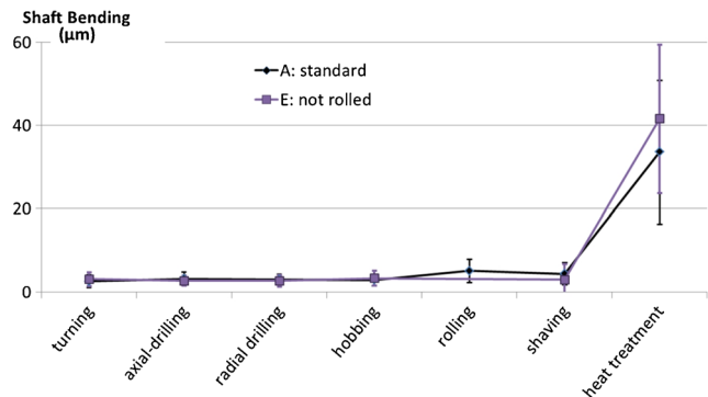
Fig. 8 Shaft bending in \infty m for two lots A and E represented with standard deviation. Lots A and E have the same manufacturing process but lot E is not rolled
