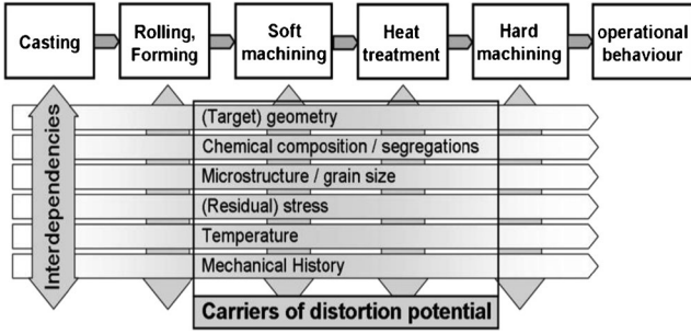
Fig. 2 Process chain and carriers of distortion potential of a typical component for the transmission industry before operational behavior [5]
