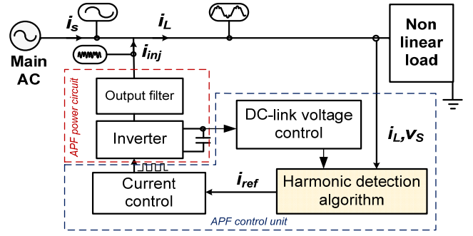
Fig. 1. A shunt APF in an electrical power system
