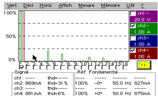
Fig.7. Spectral decomposition of the source-side current before and after compensation
