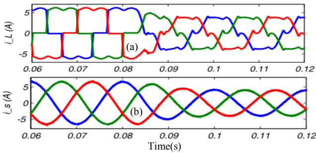
Fig. 4. Results under balanced load with a sudden change at 0.08s for mp-q, MSRF and ITM methods : (a) Load current, (b) Source currents after harmonics suppression
