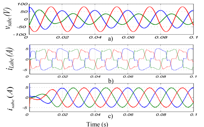
Fig. 3. Results under unbalanced and sinusoidal voltage source with balanced load for MSRF and mp-q methods: a) Unbalanced source voltage, b) Three-phase distorted load current, c) Source current after compensation
