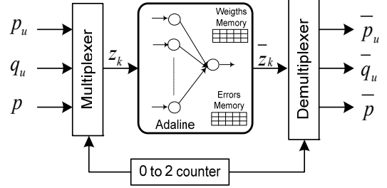
Fig. 2. Application of the multiplexing technique on the p - q harmonics detection method.
