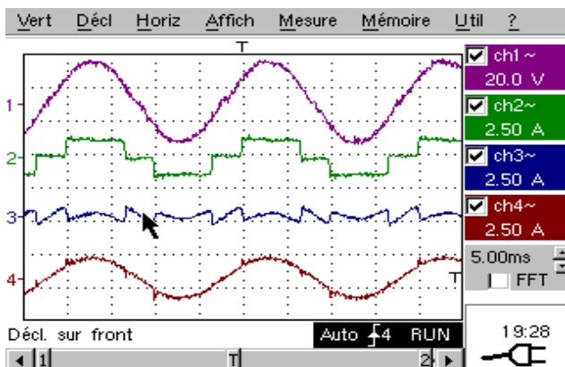
Fig.6. Experimental results for ITM and MSRF methods: 1) source voltage 2) load current 3) reference current, 4) source-side current after compensation
