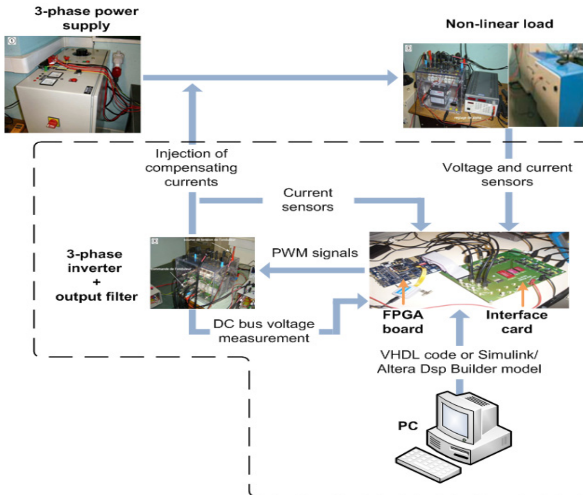
Fig. 5: Experimental principle of the APF compensation strategy.
