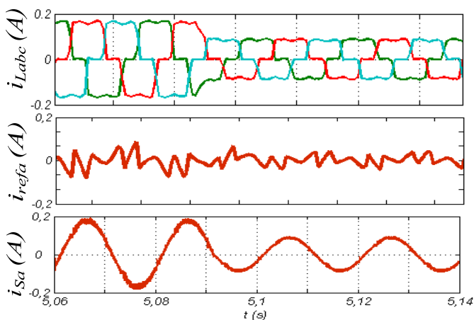
Fig. 8. Experimental results for the mp-q method - 1) three-phase load current 2) Single phase reference current, 3) source-side current after compensation
