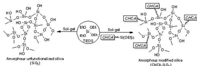
Scheme 1. Amorphous silica synthesis strategies
